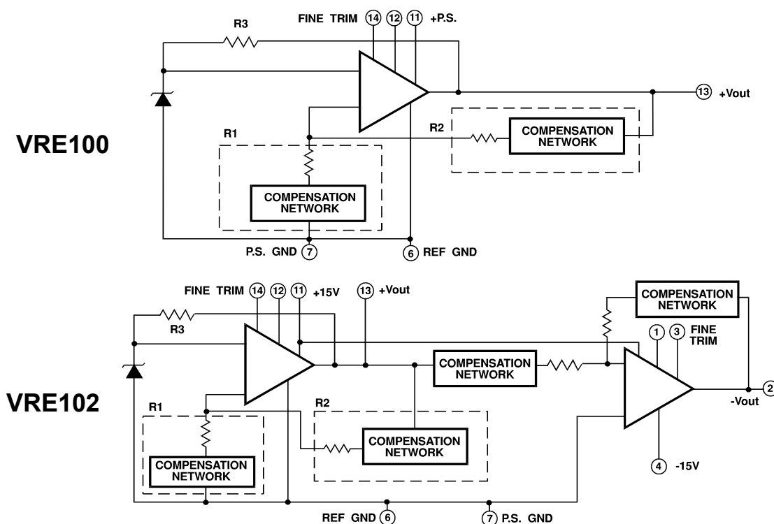
Figure 1. BLOCK DIAGRAMS
