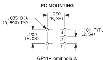
GP11MABE SPST
