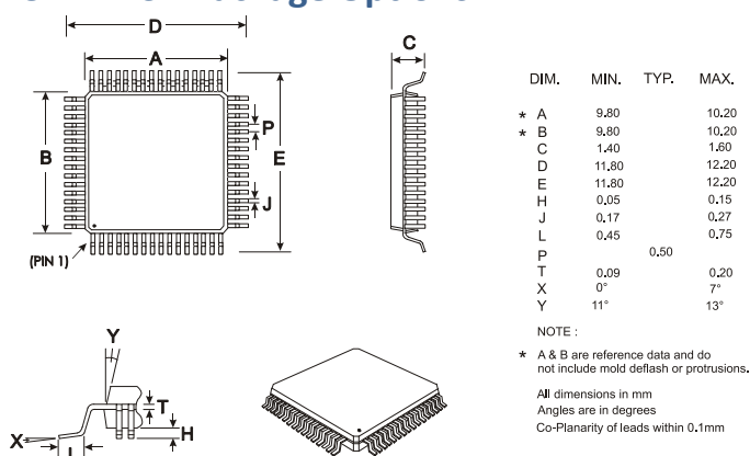
64-pin LQFP Mechanical Outline (L9)
