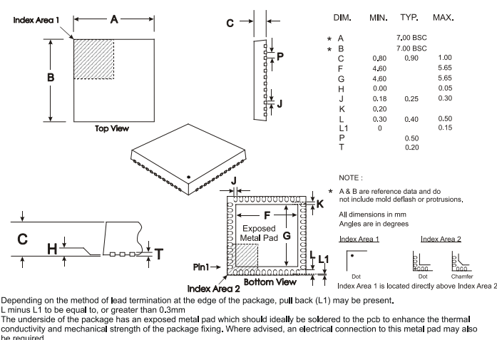
48-pin VQFN Mechanical Outline (Q3)
