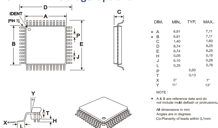
48-pin LQFP Mechanical Outline (L4)
