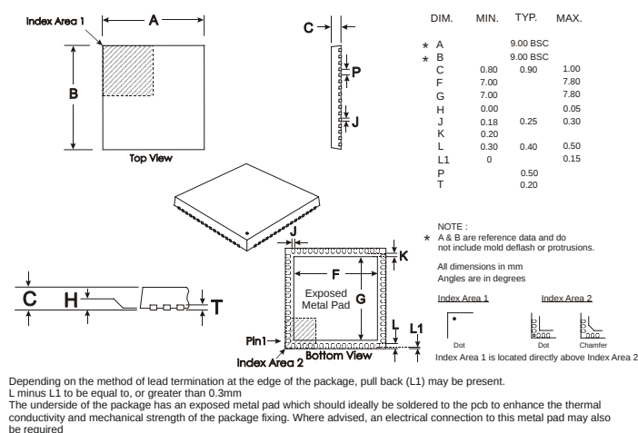
64-pin VQFN Mechanical Outline (Q1)
