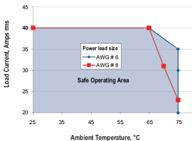
3RHPXX40XX
