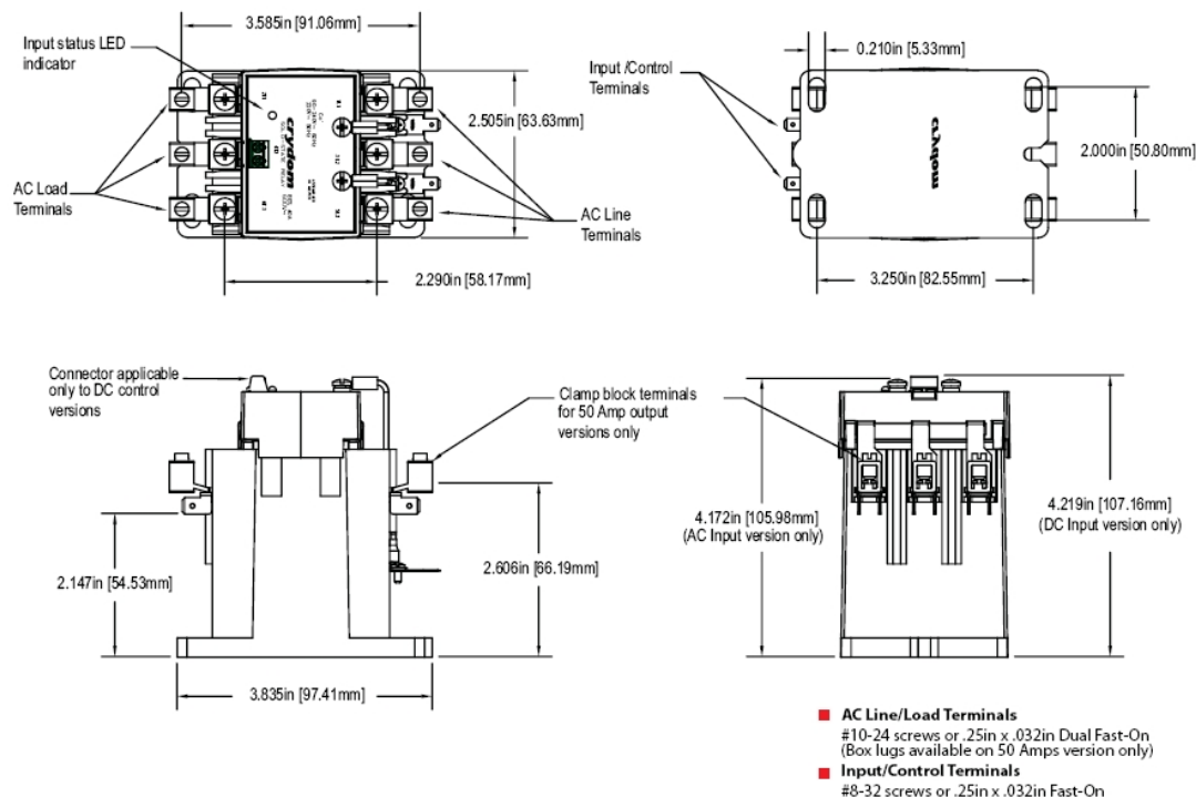
3RHPXX40XX
