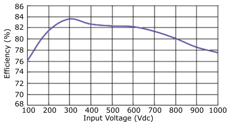
AE15-EW-S24-DIN Efficiency Curve Efficiency vs. Input Voltage
