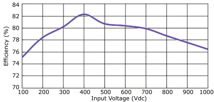
AE15-EW-S15-DIN Efficiency Curve Efficiency vs. Input Voltage
