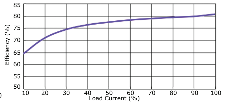
AE15-EW-S15-DIN Efficiency Curve Efficiency vs. Load Current
