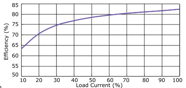
AE15-EW-S24-DIN Efficiency Curve Efficiency vs. Load Current
