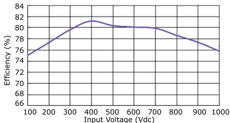
AE15-EW-S12-DIN Efficiency Curve Efficiency vs. Input Voltage
