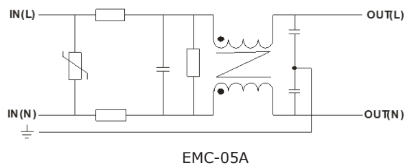
Figure 1 Internal Circuit
