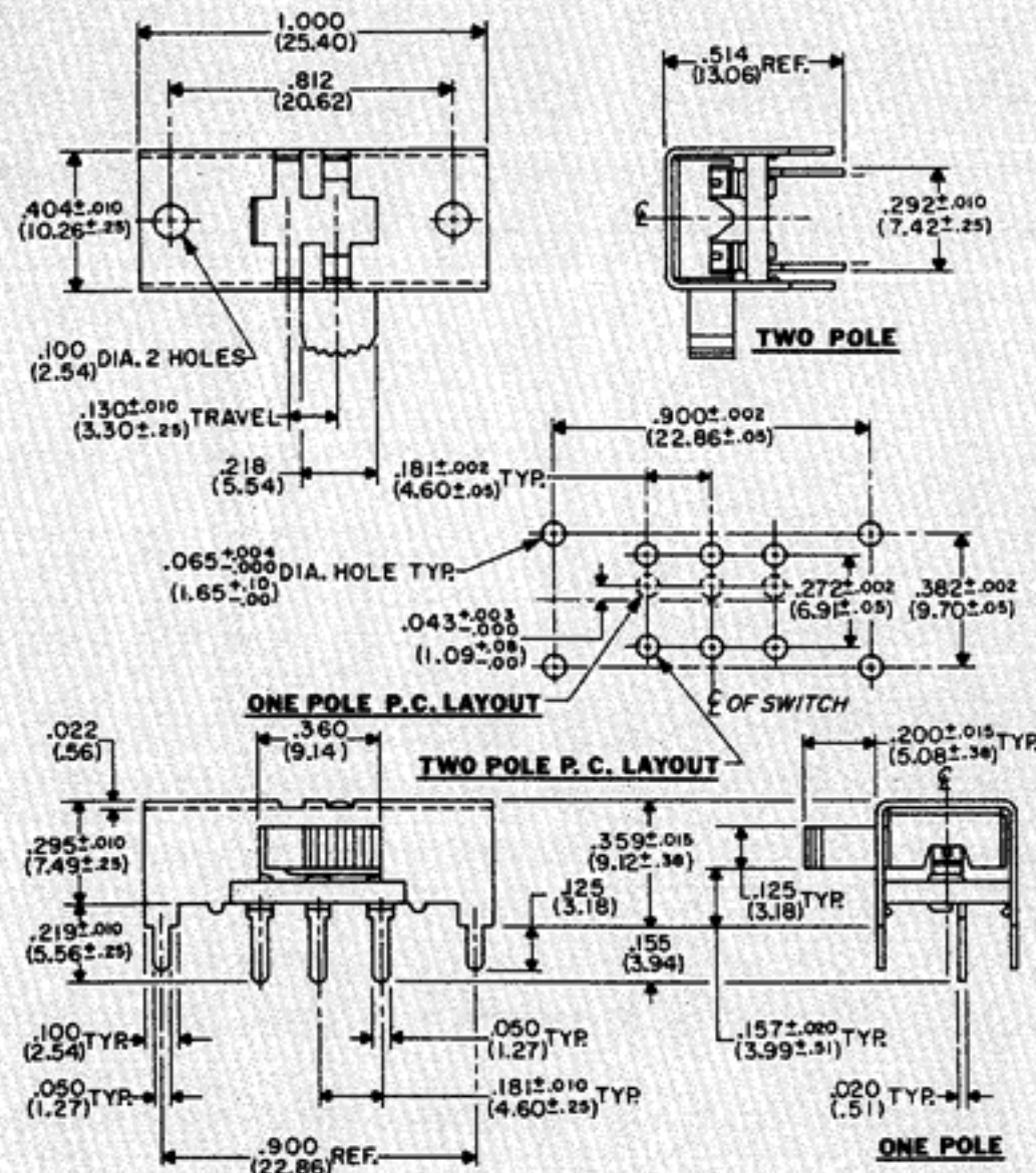
GPI-151 Single Pole Double Throw (with detent) GPI-152 Double Pole Double Throw (with detent)
