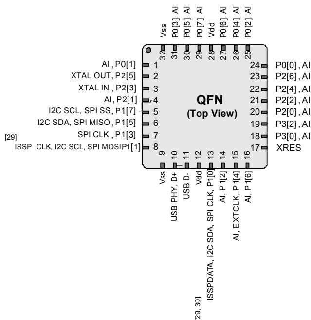
Figure 8. CY8C20496A
