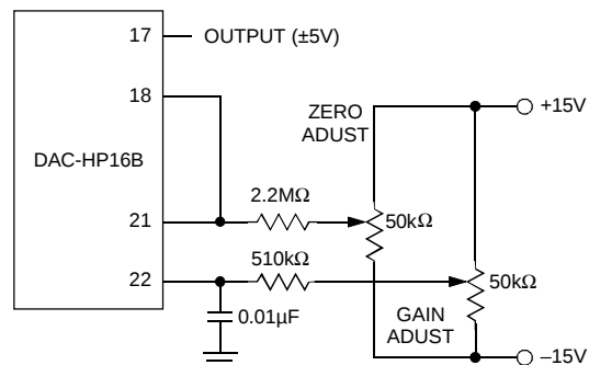
Figure 4. Bipolar Operations
