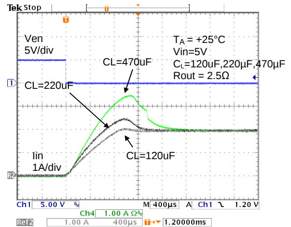
Inrush Current
