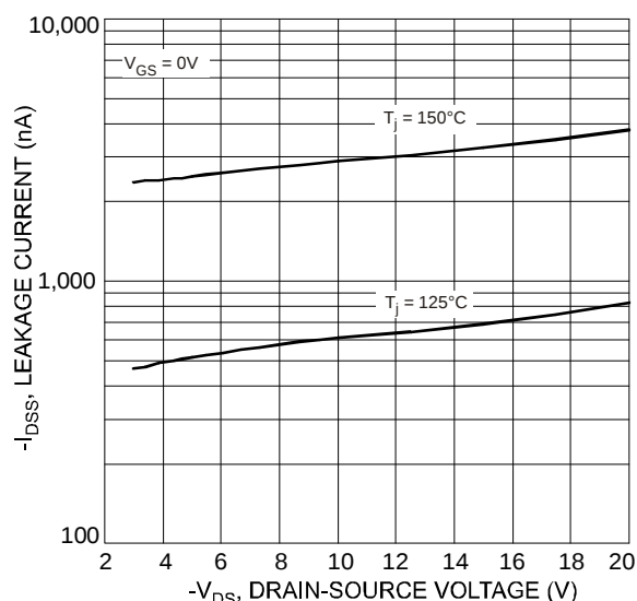
Fig. 8 Drain-Source Leakage Current vs Voltage
