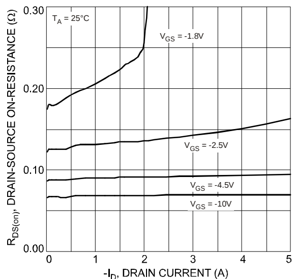
Fig. 4 On-Resistance vs Drain Current and Gate Voltage
