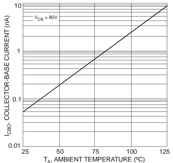
Fig. 6 Typical Collector-Cutoff Current vs. Ambient Temperature
