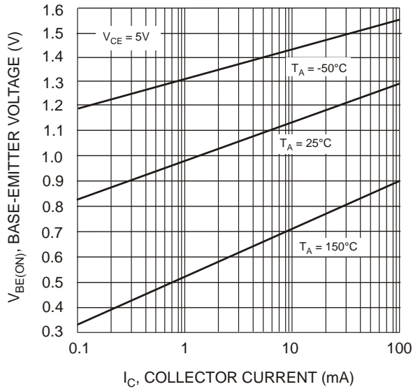
Fig. 3 Typical Base-Emitter Voltage vs. Collector Current
