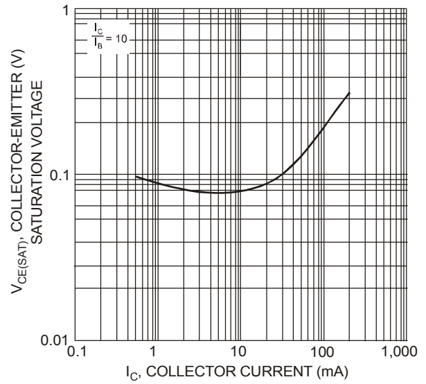
Fig. 8, Typical Collector-Emitter Saturation Voltage vs. Collector Current (NPN-4124)
