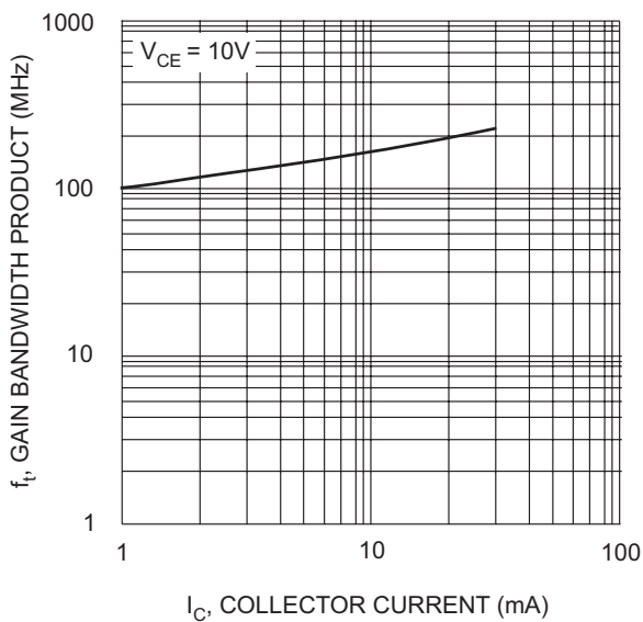
I_C , COLLECTOR CURRENT (mA) Fig. 9, Gain Bandwidth Product vs Collector Current (PNP5401)
