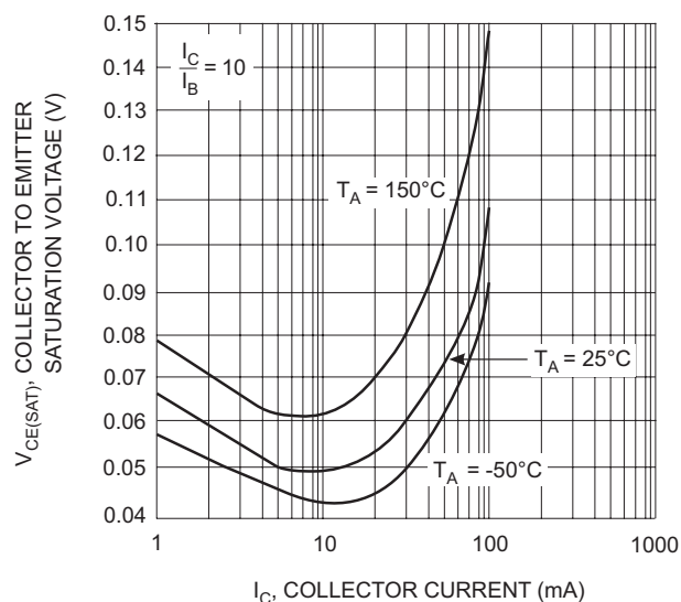
Fig. 2, Collector Emitter Saturation Voltage vs. Collector Current (NPN5551)
