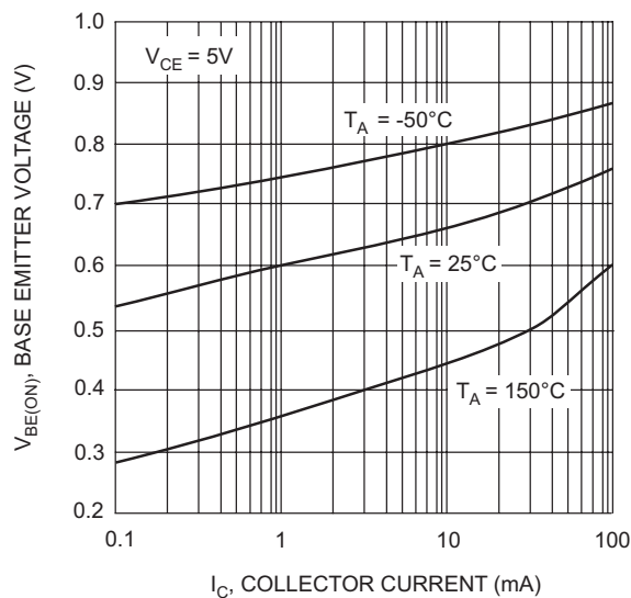
Fig. 4, Base Emitter Voltage vs. Collector Current (NPN5551)
