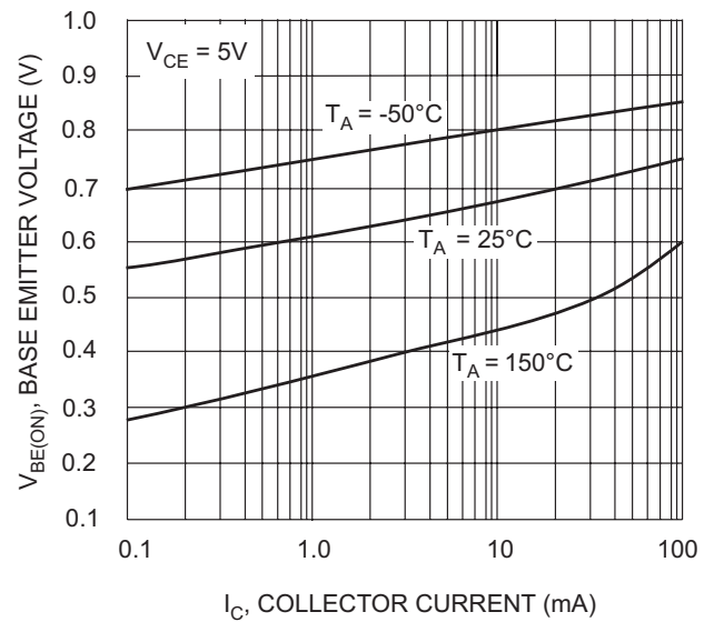
I_C , COLLECTOR CURRENT (mA) Fig. 8, Base Emitter Voltage vs. Collector Current (PNP5401)
