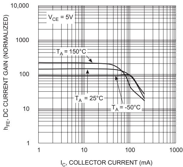
I_C , COLLECTOR CURRENT (mA) Fig. 7, DC Current Gain vs. Collector Current (PNP5401)
