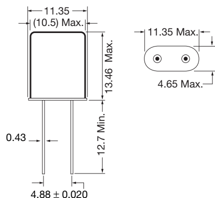
Figure 1) HC-49UX - Side and Bottom views
