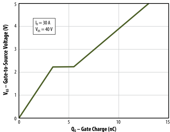
Figure 6: Gate Charge
