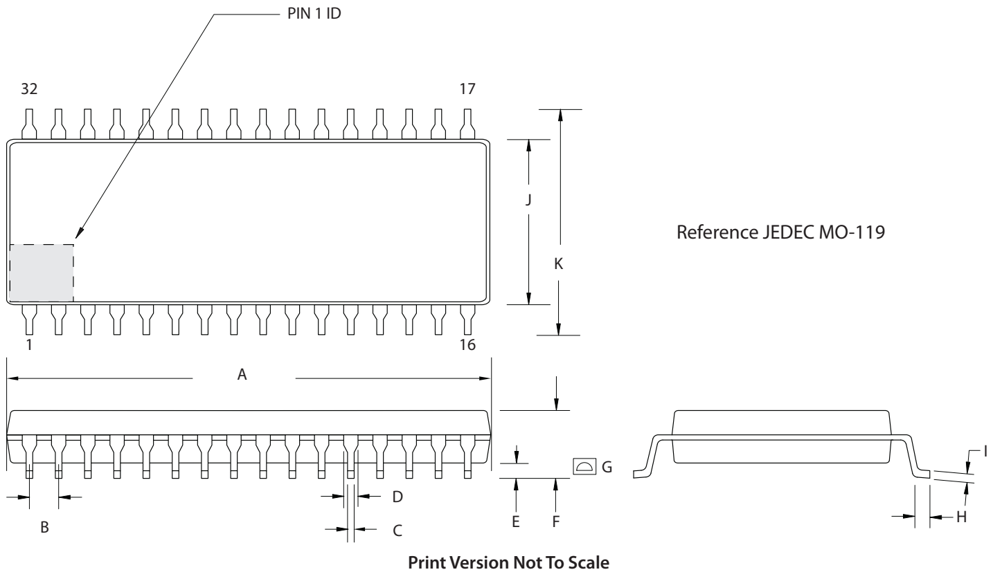
Figure 5.3 SOIC
