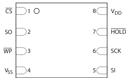
8-Pin DFN or 8-Pin DFN Small Flag Packages
