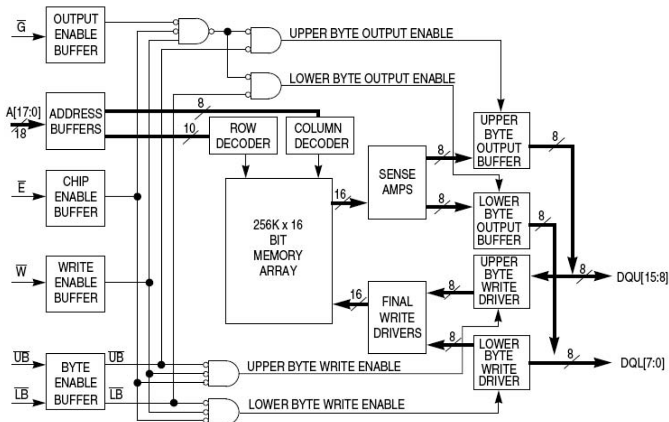
Figure 1.1 Block Diagram
