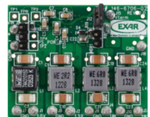
Zynq-7000 Power System Featuring XRP7714
