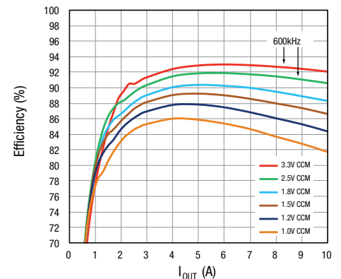
f = 500\text{kHz} , V_{IN} = 12\text{V} XR79110 Efficiency
