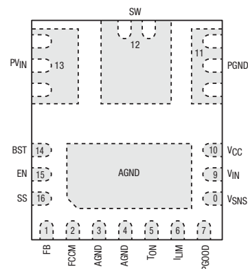
XR76120 Pin Assignment
