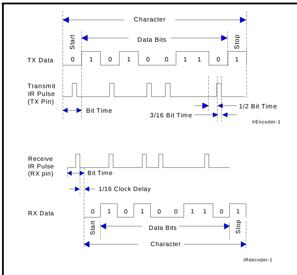
FIGURE 15. INFRARED TRANSMIT DATA ENCODING AND RECEIVE DATA DECODING
