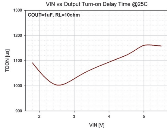
Fig. 17: Output Turn-On Delay Time vs. Input Voltage
