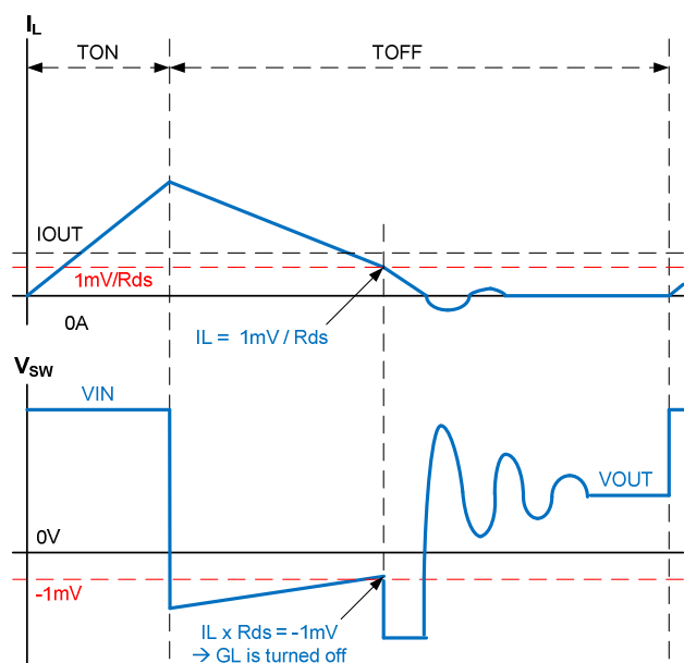
Figure 30. Discontinuous conduction during diode emulation
