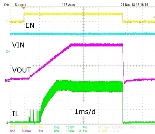
Fig. 21: Enable turn on/turn off, 12V IN , 1.2V OUT , 25A
