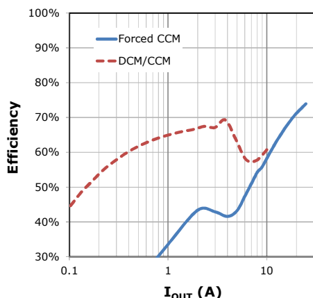
Fig. 20: Efficiency, 20V IN , 1.2V OUT , 1uH, 300kHz
