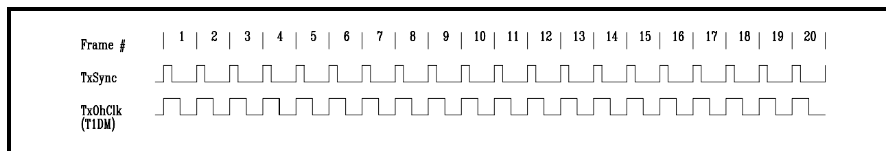
FIGURE 33. DS1 TRANSMIT OVERHEAD INPUT INTERFACE MODULE IN T1DM FRAMING FORMAT MODE
