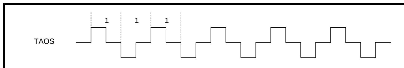
FIGURE 42. TAOS (TRANSMIT ALL ONES)
