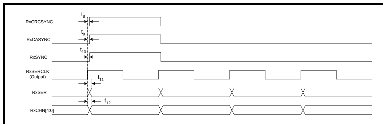
FIGURE 107. FRAMER SYSTEM RECEIVE TIMING DIAGRAM (RxSERCLK AS AN OUTPUT)
