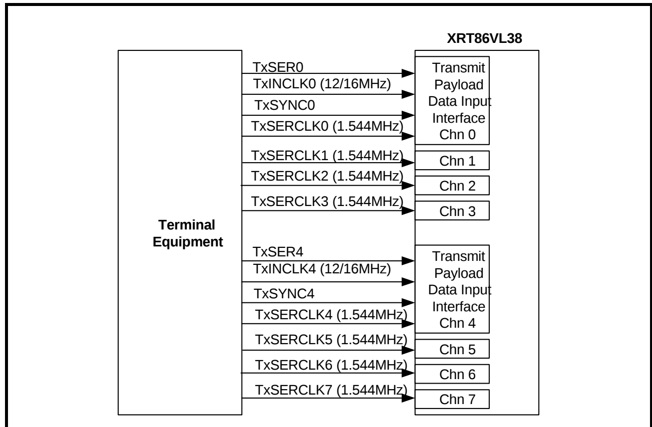
FIGURE 81. INTERFACING XRT86VL3X TRANSMIT TO LOCAL TERMINAL EQUIPMENT USING 16.384MBIT/S, HMVIP 16.384MBIT/S, AND H.100 16.384MBIT/S
