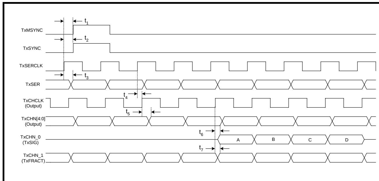
FIGURE 106. FRAMER SYSTEM TRANSMIT TIMING DIAGRAM (BASE RATE/NON-Mux)
