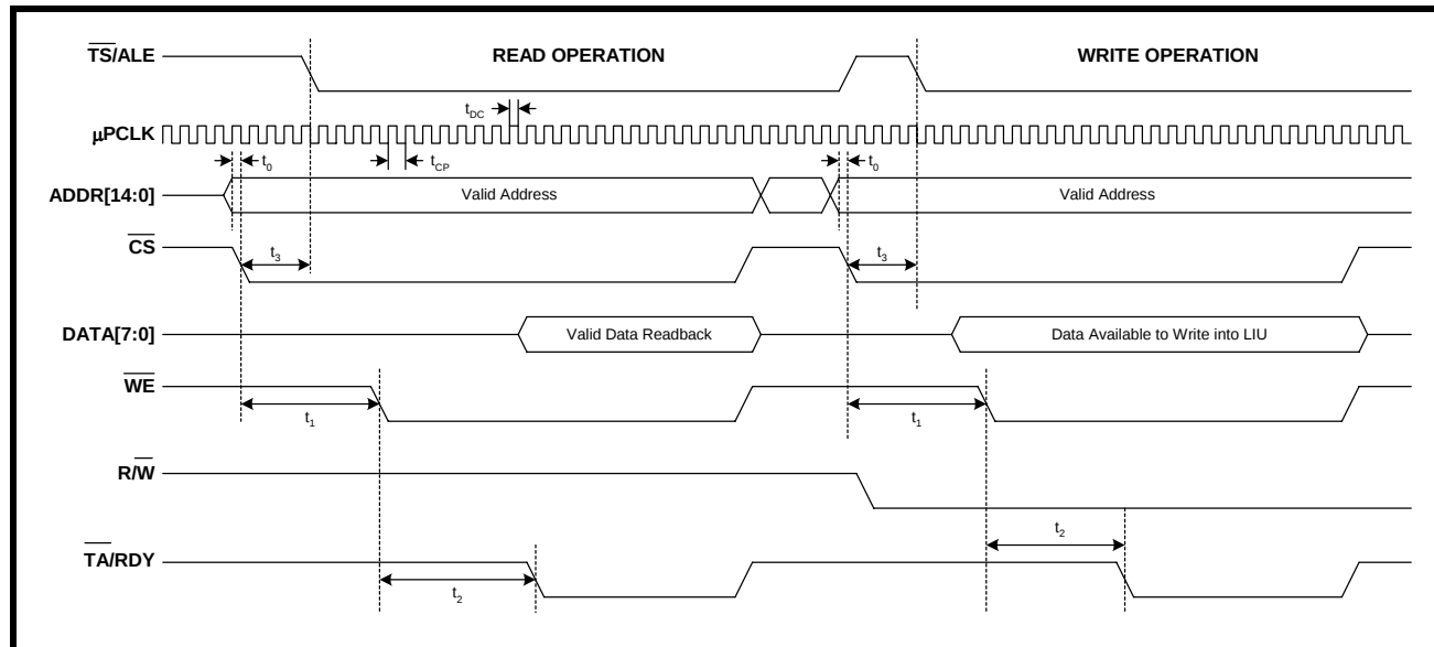
FIGURE 119. POWER PC 403 INTERFACE SIGNALS DURING PROGRAMMED I/O READ AND WRITE OPERATIONS
