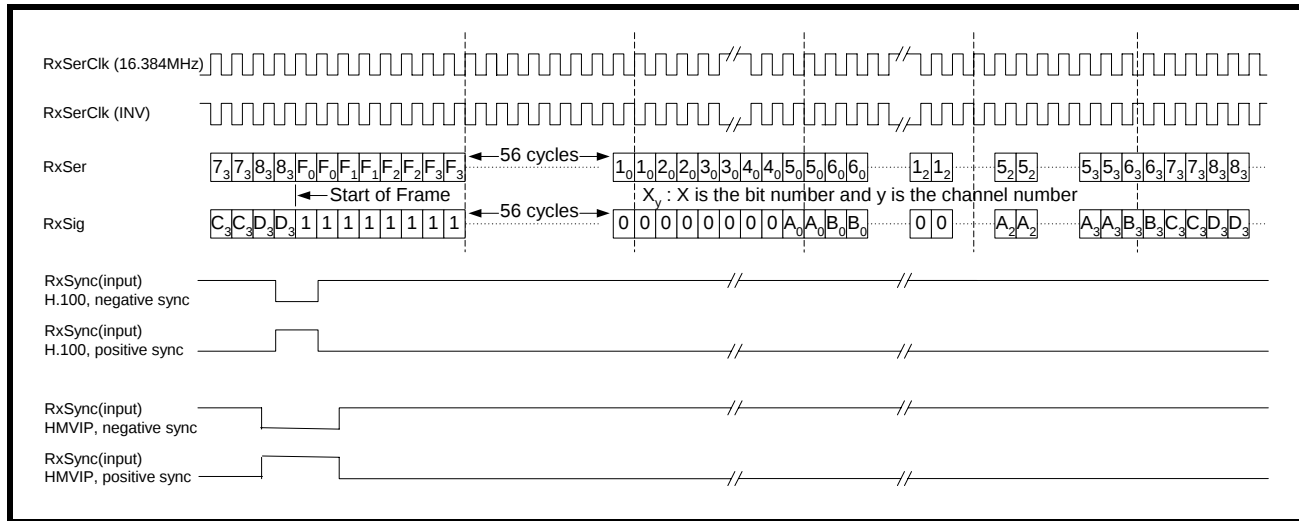
FIGURE 88. WAVEFORMS FOR CONNECTING THE RECEIVE MULTIPLEXED HIGH-SPEED INPUT INTERFACE AT HMVIP AND H.100 16.384MBIT/S MODE
