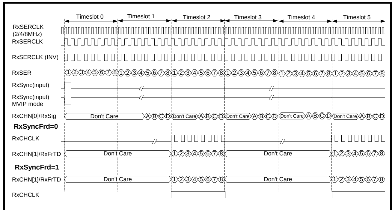
FIGURE 64. WAVEFORMS FOR CONNECTING THE RECEIVE NON-MULTIPLEXED HIGH-SPEED INPUT INTERFACE AT MVIP 2.048Mbit/s, 4.096Mbit/s, AND 8.192Mbit/s
