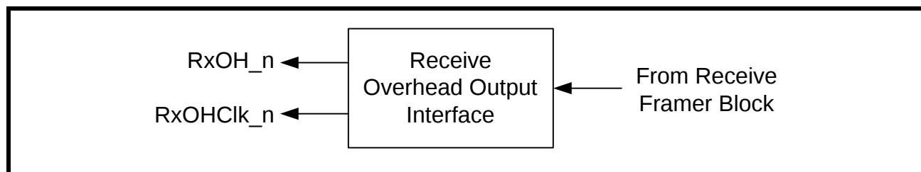
FIGURE 34. BLOCK DIAGRAM OF THE DS1 RECEIVE OVERHEAD OUTPUT INTERFACE OF XRT86VL3X
