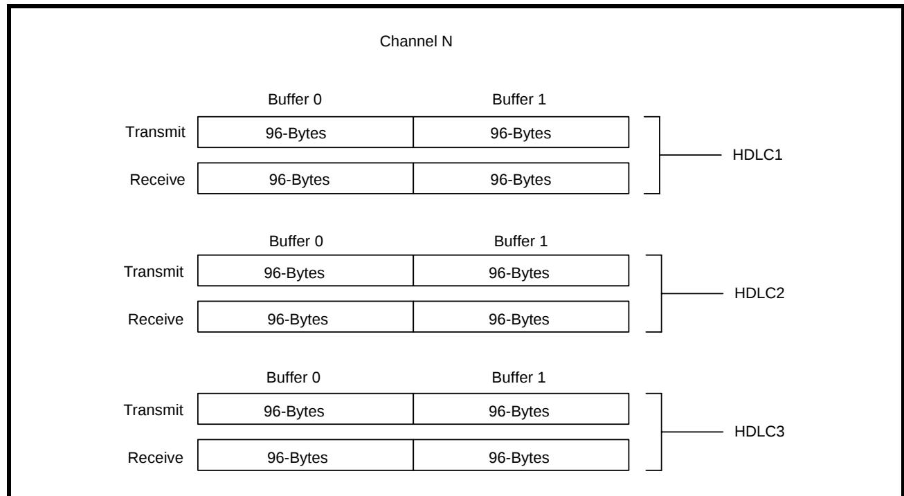
FIGURE 28. HDLC CONTROLLERS
