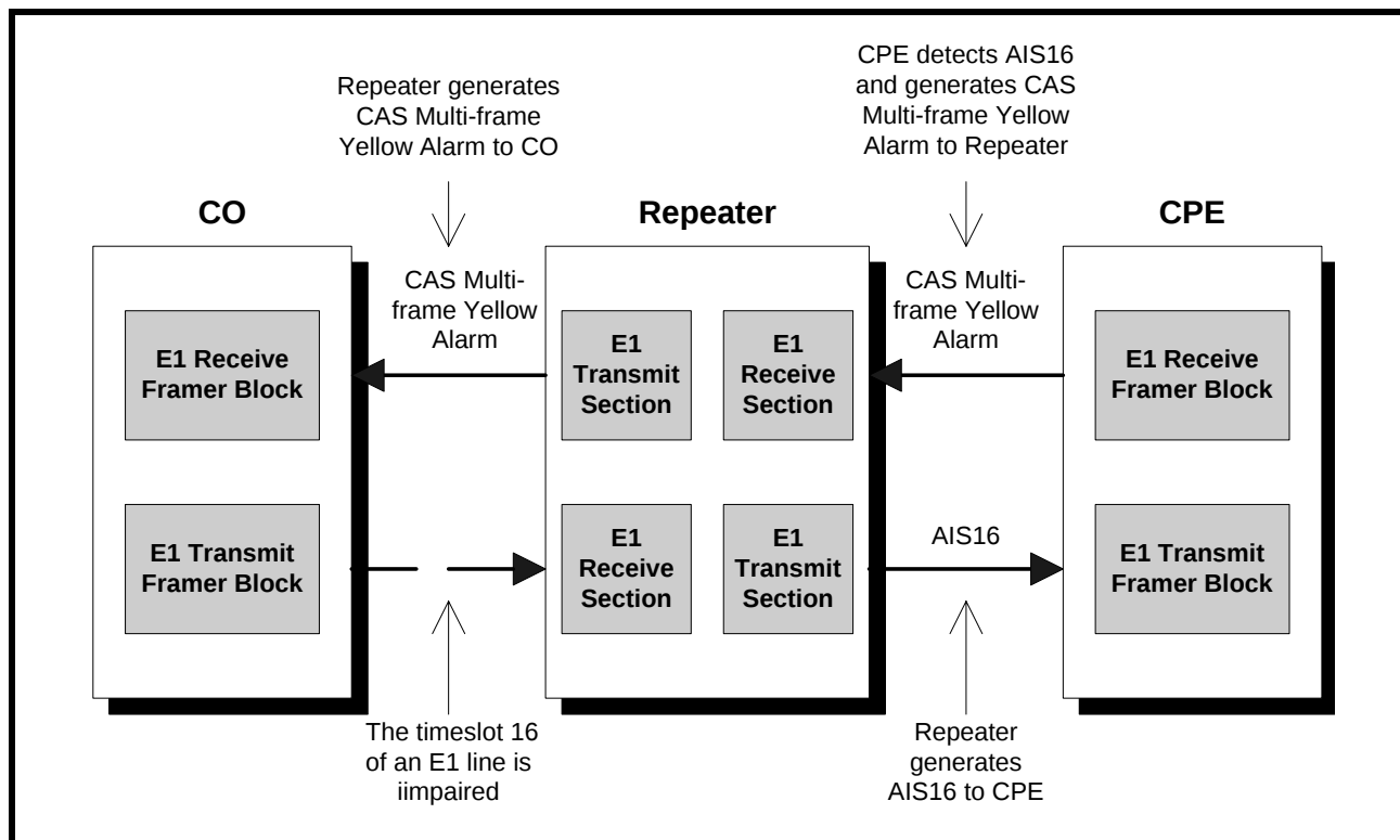
FIGURE 95. GENERATION OF CAS MULTI-FRAME YELLOW ALARM BY THE CPE UPON DETECTION OF "AIS16" PATTERN SENT BY THE REPEATER
