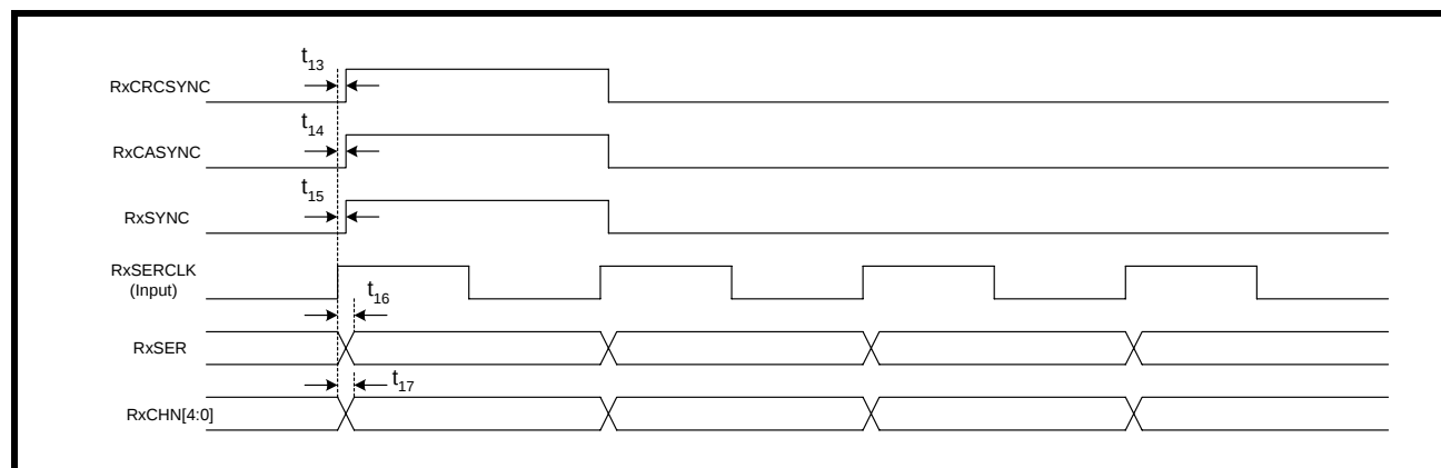
FIGURE 108. FRAMER SYSTEM RECEIVE TIMING DIAGRAM (RxSERCLK AS AN INPUT)
