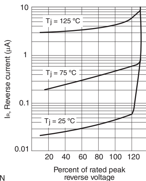
TYPICAL REVERSE CHARACTERISTIC
