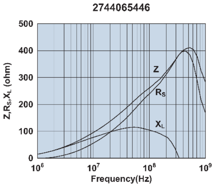
Impedance, reactance, and resistance vs. frequency.
