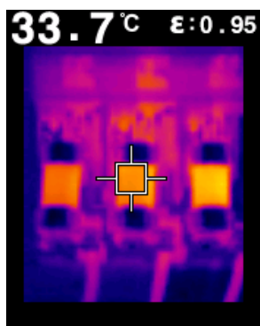
Electrical Troubleshooting
