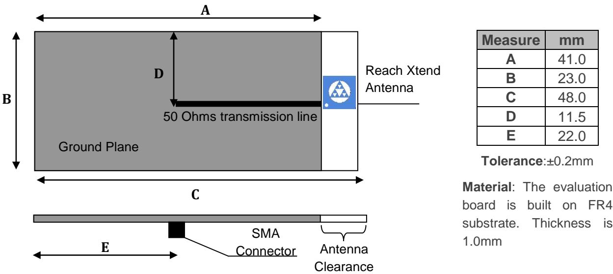
Figure 1 – EB_FR05-S1-N-0-001. Reach Xtend™ Evaluation Board.
