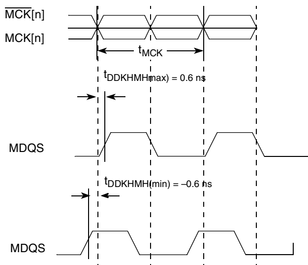
Figure 5. Timing Diagram for t_{DPKHMH}
