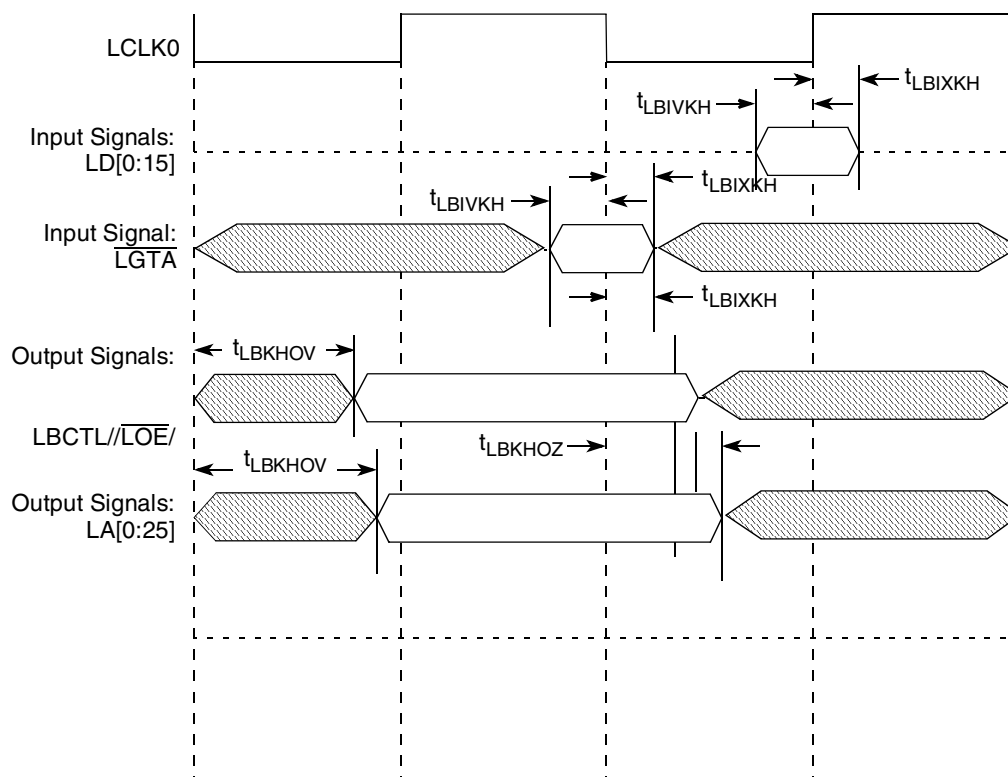
Figure 31. Local Bus Signals, Non-Special Signals Only
