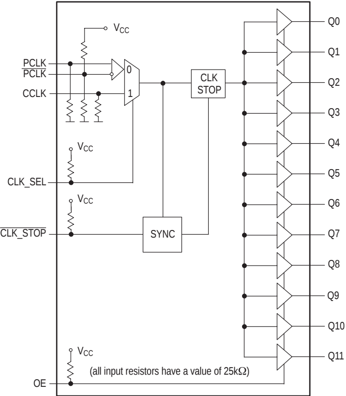
Figure 1. Logic Diagram
