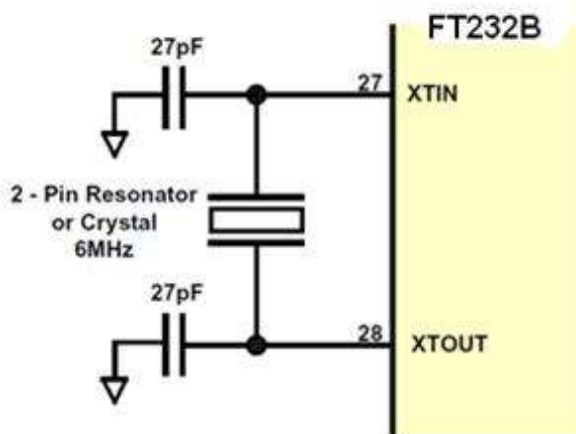
Figure 7.2 Crystal or 2 Pin Ceramic Resonator Configuration
