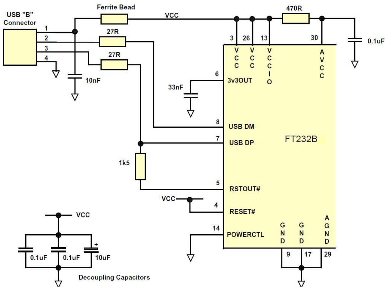
Figure 6.1 Bus Powered Configuration
