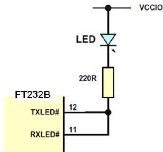
Figure 9.2 Single LED
