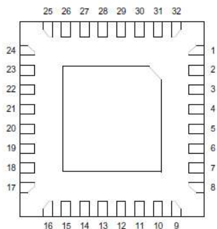
Pin-Out (QFN32 Package )
