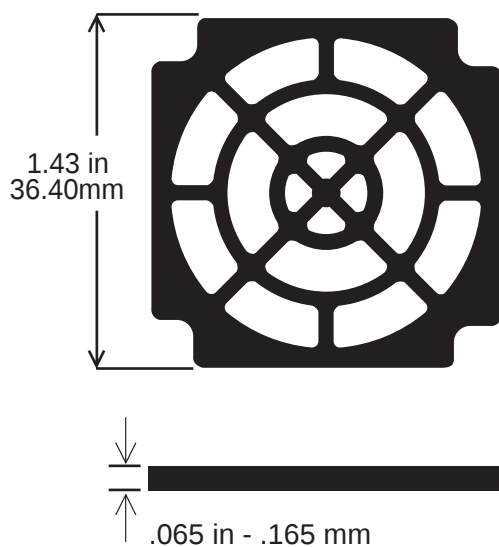
SC40-P05 Retainer
