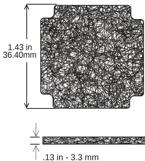
SC40-M45 Filter
