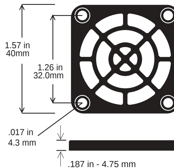
SC40-P10 Guard
