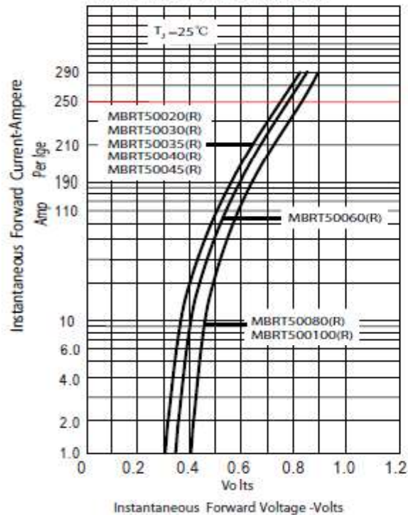
Figure.1-Typical Forward Characteristics
