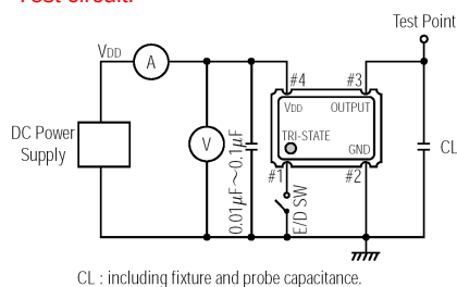
Test circuit:
