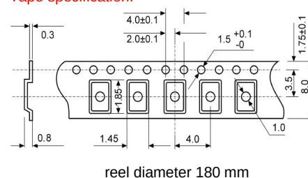
Tape specification:
