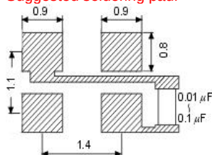
Suggested soldering pad:
