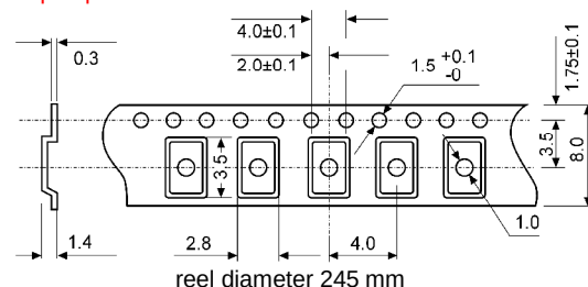
Tape specification:
