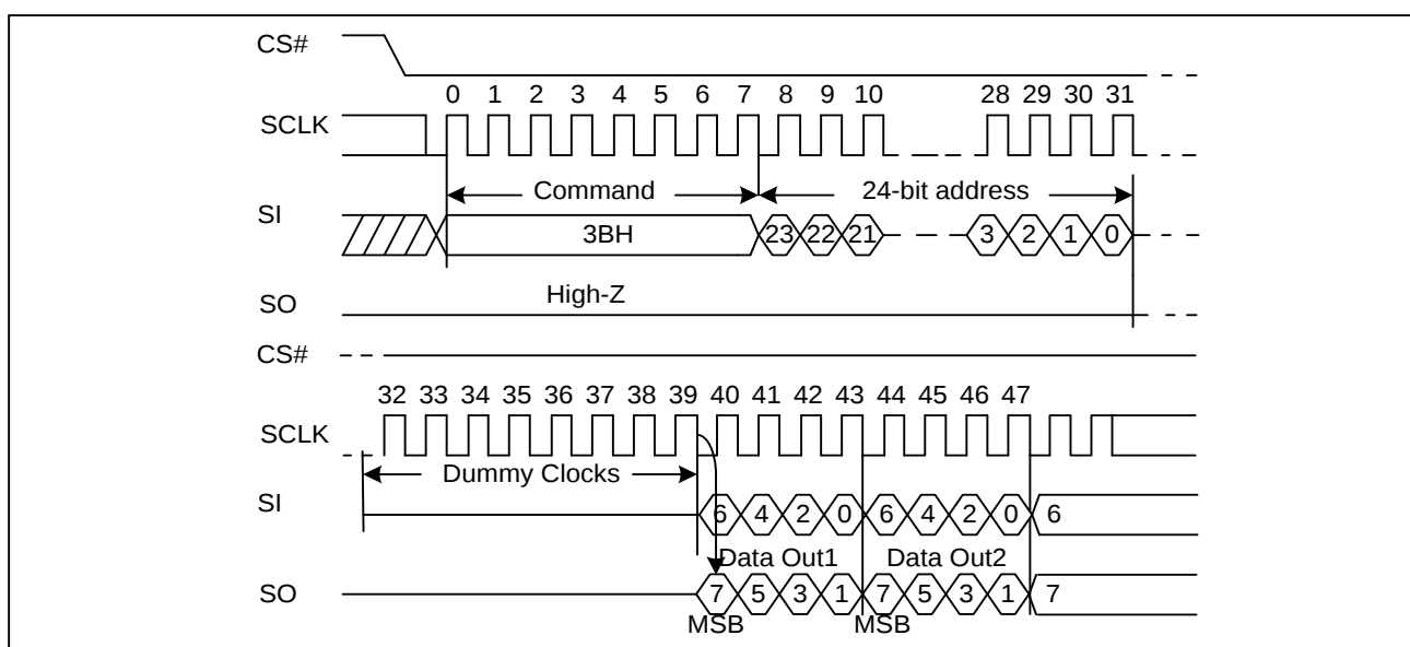
Figure9. Dual Output Fast Read Sequence Diagram
