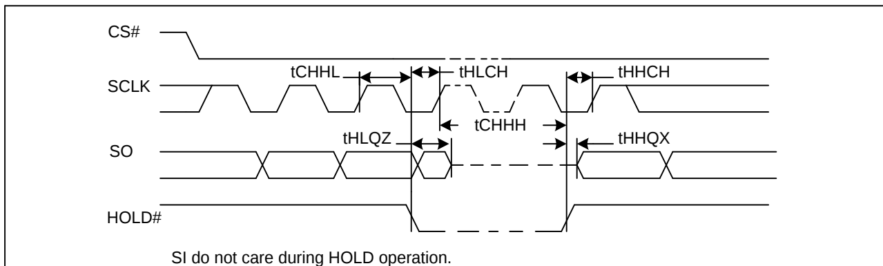
Figure44. Hold Timing
