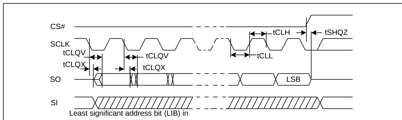
Figure40. Output Timing
