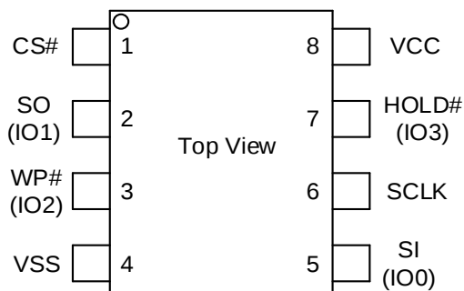
8 - LEAD VSOP/SOP
