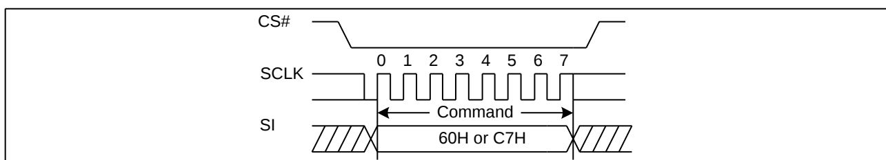
Figure19. Chip Erase Sequence Diagram
