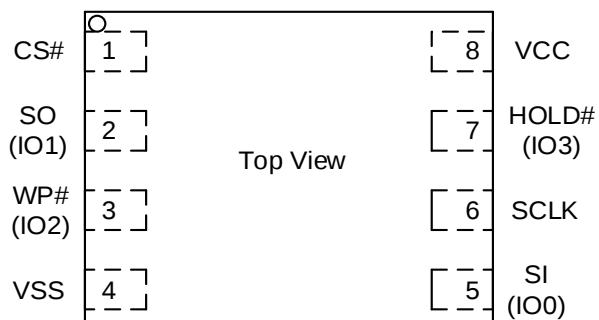
8 - LEAD WSON/USON/LGA
