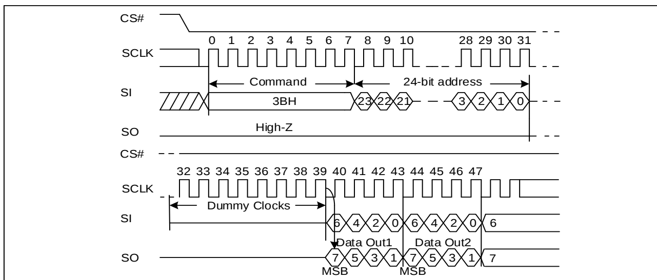
Figure9. Dual Output Fast Read Sequence Diagram
