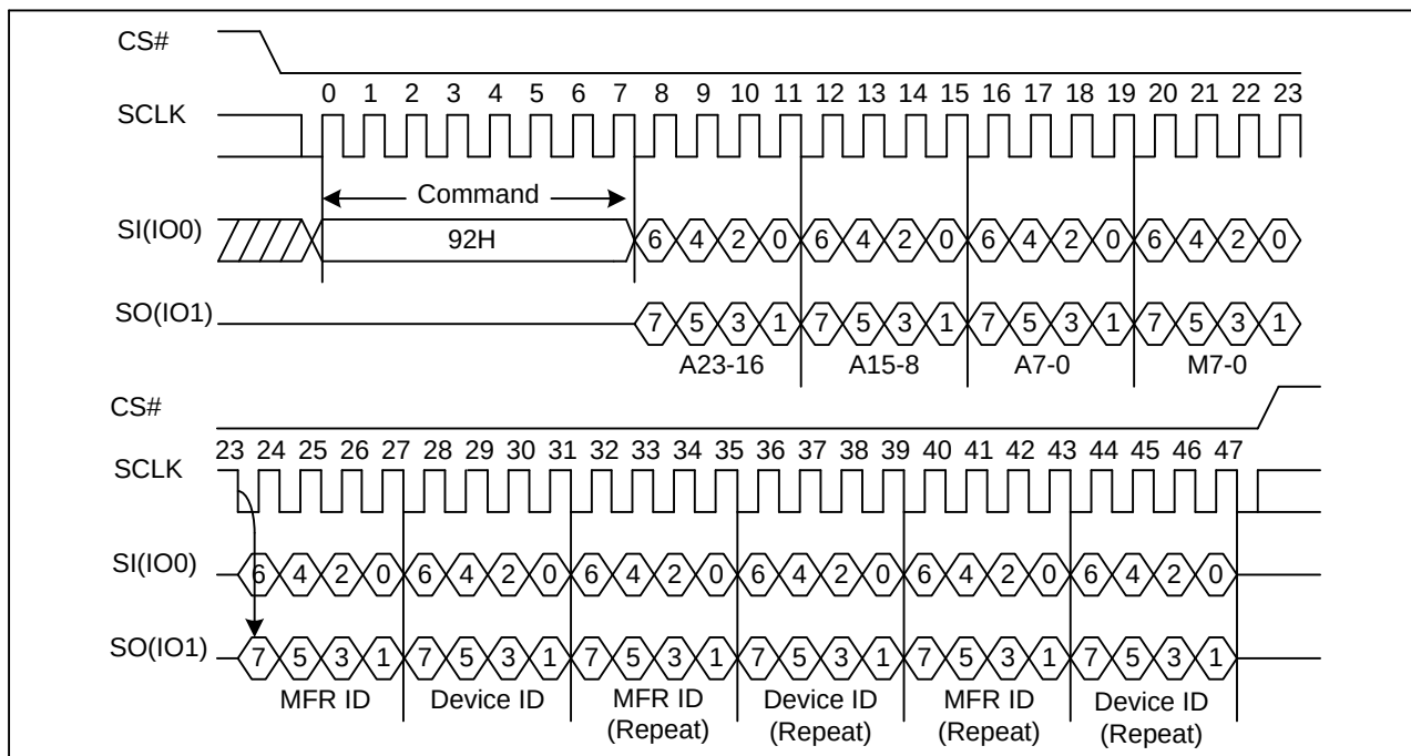
Figure28. Read Manufacturer ID/ Device ID Dual I/O Sequence Diagram
