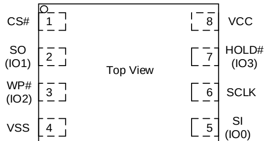
8 - LEAD WSON/USON/LGA
