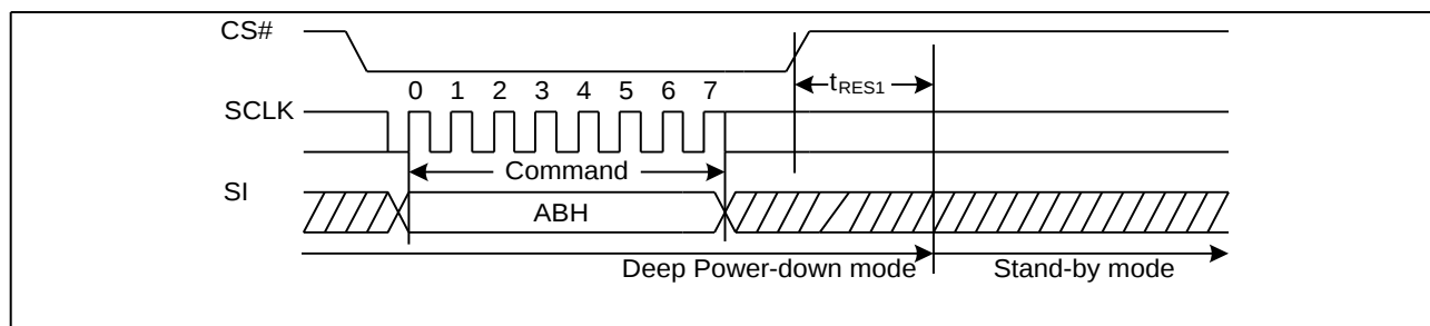
Figure24. Release Power-Down/Read Device ID Sequence Diagram
