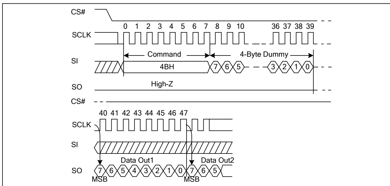
Figure35 Read Unique ID Sequence Diagram
