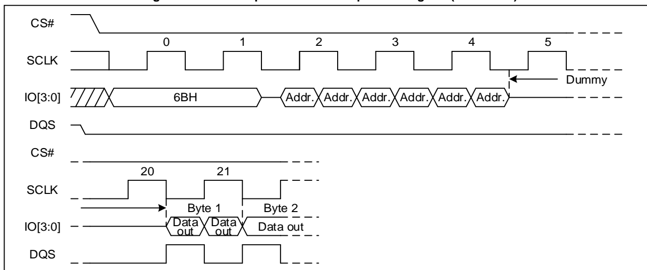
Figure 48 Quad Output Fast Read Sequence Diagram (Quad DTR)
