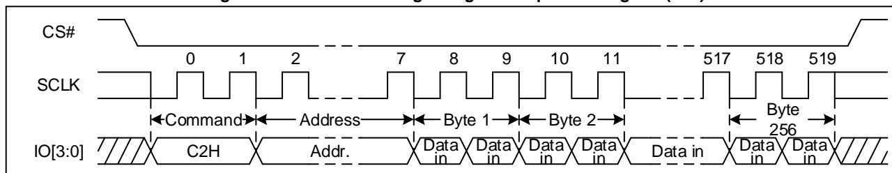
Figure 65 Extend Quad Page Program Sequence Diagram (QPI)
