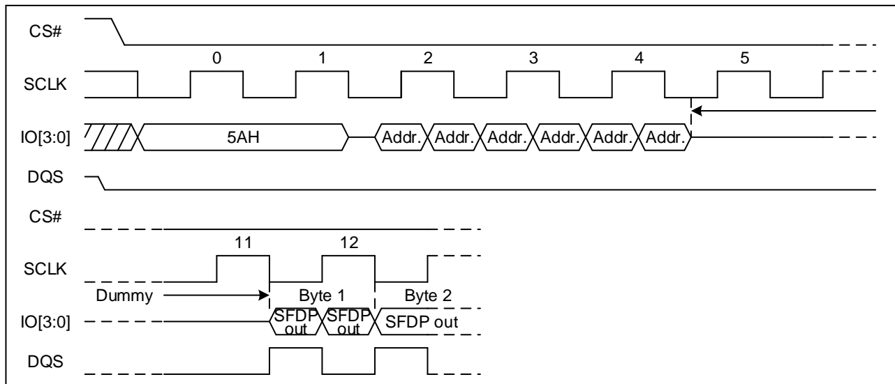
Figure 122 Read Serial Flash Discoverable Parameter command Sequence Diagram (DTR, QPI)
