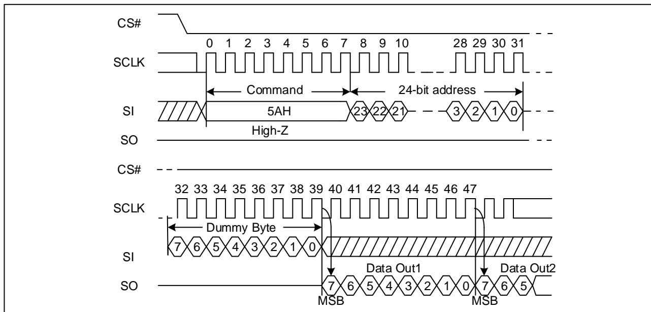
Figure 120 Read Serial Flash Discoverable Parameter command Sequence Diagram (SPI)
