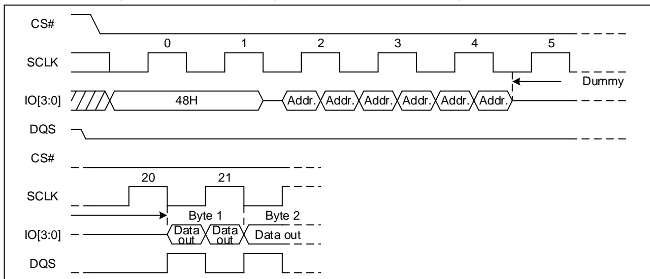
Figure 104 Read Security Registers command Sequence Diagram (Quad DTR)
