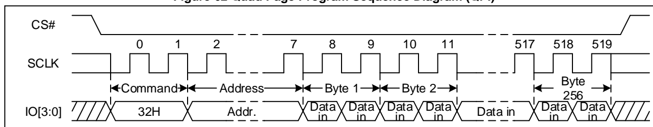
Figure 62 Quad Page Program Sequence Diagram (QPI)
