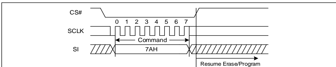
Figure 94 Program/Erase Resume Sequence Diagram
