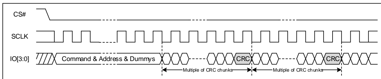
Figure 3. CRC Timing
