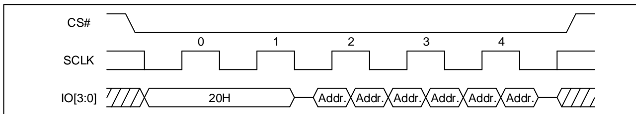
Figure 69 Sector Erase Sequence Diagram (Quad DTR)
