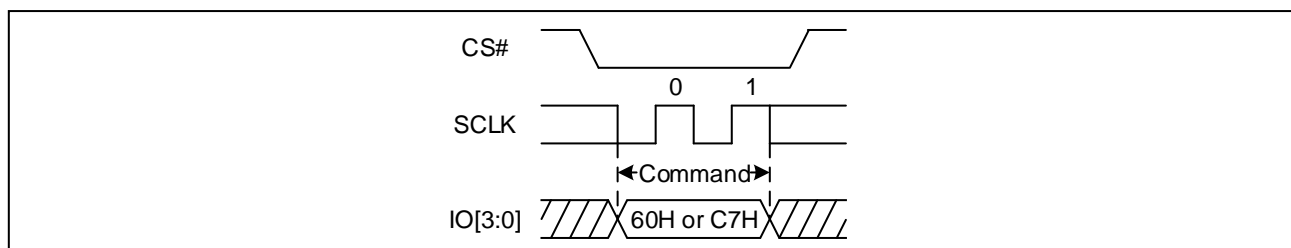
Figure 77 Chip Erase Sequence Diagram (QPI &amp; Quad DTR)
