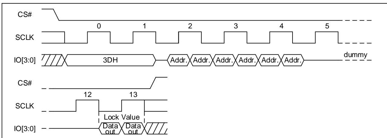
Figure 113 Read Individual Block/Sector lock command Sequence Diagram (Quad DTR)
