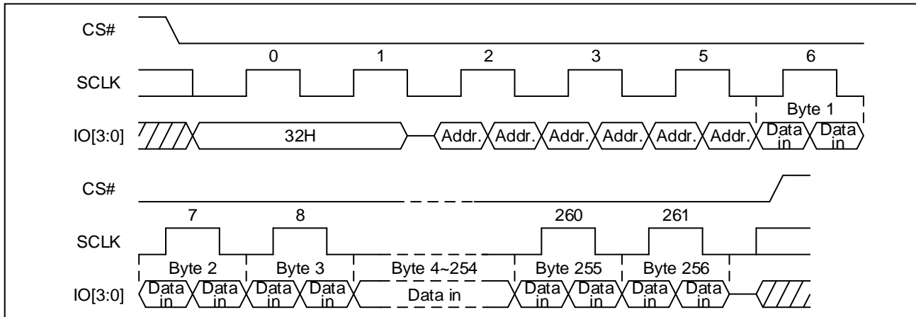
Figure 63 Quad Page Program Sequence Diagram (Quad DTR)
