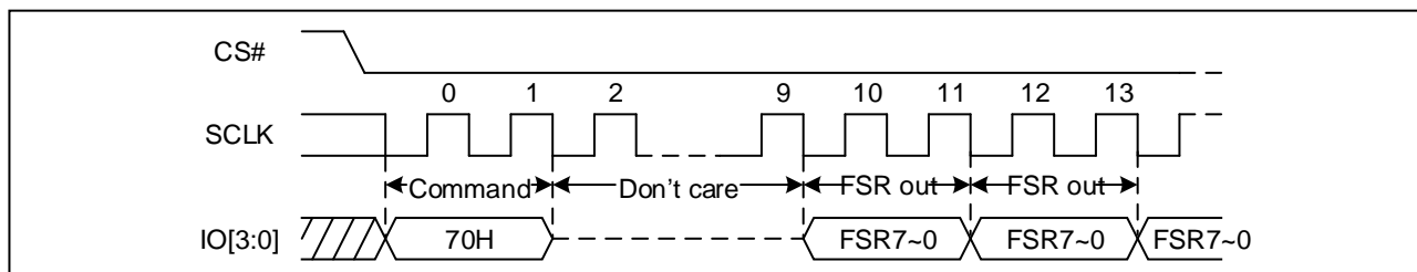
Figure 33 Read Flag Status Register Sequence Diagram (QPI, fSCLK &gt; 104MHz)
