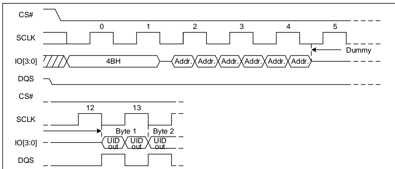
Figure 87 Read Unique ID Sequence Diagram (Quad DTR)
