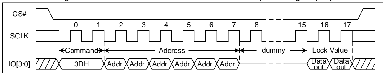
Figure 112 Read Individual Block/Sector lock command Sequence Diagram (QPI)
