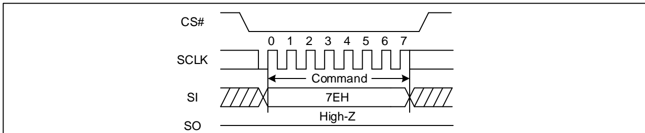
Figure 114 Global Block/Sector Lock Sequence Diagram (SPI)
