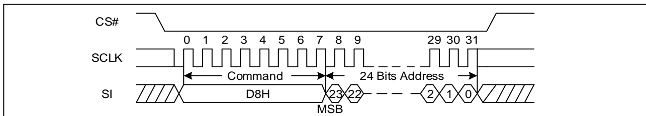
Figure 73 64KB Block Erase Sequence Diagram (SPI)
