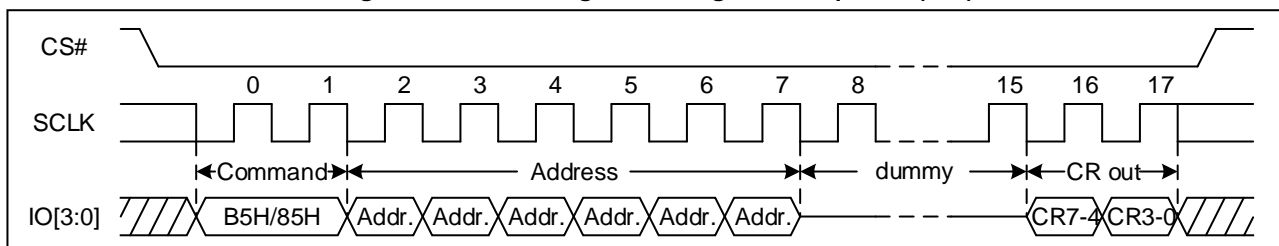
Figure 36 Read Configuration Registers Sequence (QPI)
