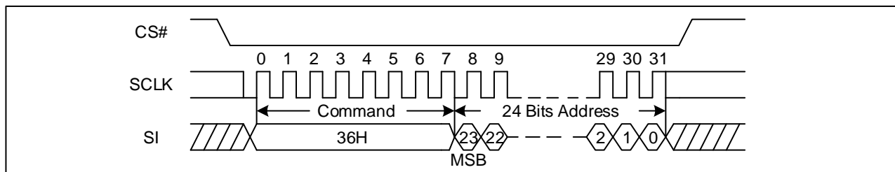
Figure 105 Individual Block/Sector Lock command Sequence Diagram (SPI)
