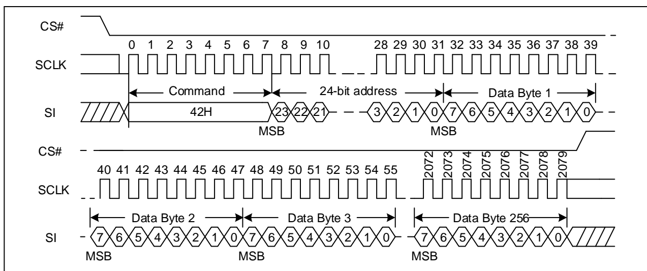
Figure 99 Program Security Registers command Sequence Diagram (SPI)
