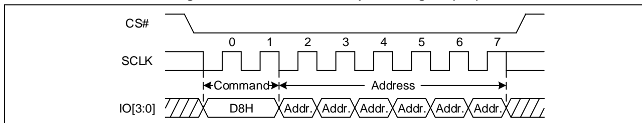
Figure 74 64KB Block Erase Sequence Diagram (QPI)
