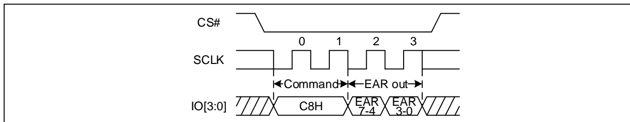
Figure 40 Read Extended Address Register Sequence Diagram (QPI, f_{SCLK} > 104\text{MHz} )
