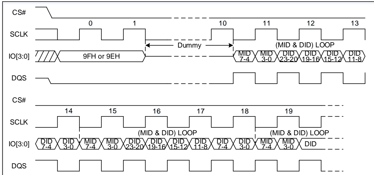
Figure 91 Read Identification ID Sequence Diagram (Quad DTR)
