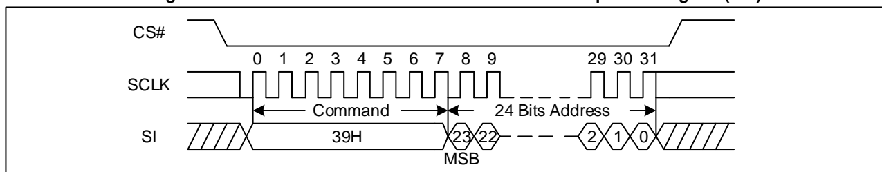
Figure 108 Individual Block/Sector Unlock command Sequence Diagram (SPI)
