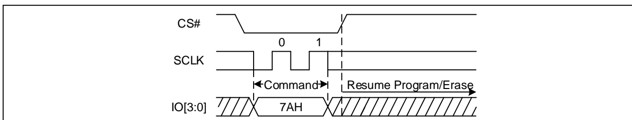
Figure 95 Program/Erase Resume Sequence Diagram (QPI & Quad DTR)
