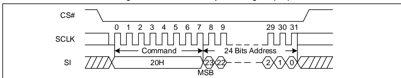
Figure 67 Sector Erase Sequence Diagram (SPI)
