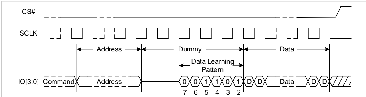
Figure 7. Data Learning Pattern Sequence Diagram (DTR, Dummy Clock &lt; 6)
