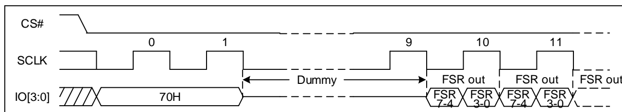
Figure 34 Read Flag Status Register Sequence Diagram (Quad DTR)
