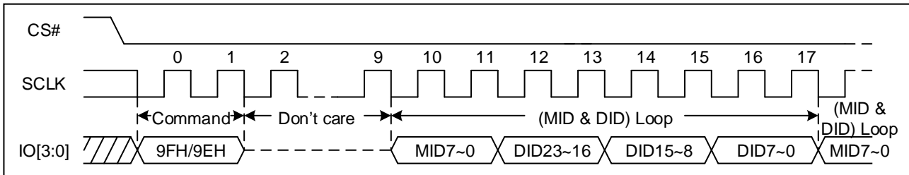
Figure 90 Read Identification ID Sequence Diagram (QPI, f_{SCLK} > 104\text{MHz} )
