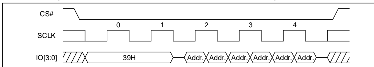
Figure 110 Individual Block/Sector Unlock command Sequence Diagram (Quad DTR)
