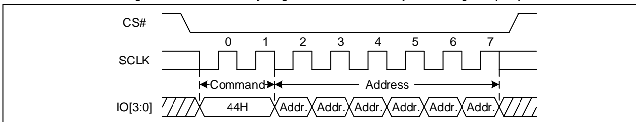
Figure 97 Erase Security Registers command Sequence Diagram (QPI)
