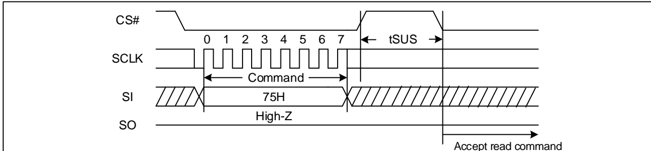
Figure 92 Program/Erase Suspend Sequence Diagram (SPI)
