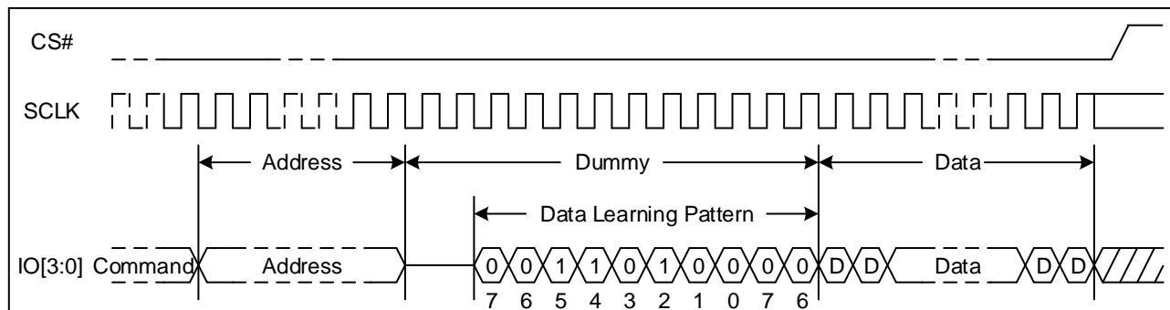
Figure 4. Data Learning Pattern Sequence Diagram (STR, Dummy Clock \geq 10 )
