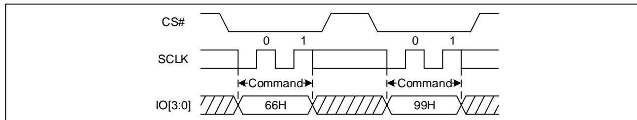
Figure 119 Enable Reset and Reset command Sequence Diagram (QPI & Quad DTR)
