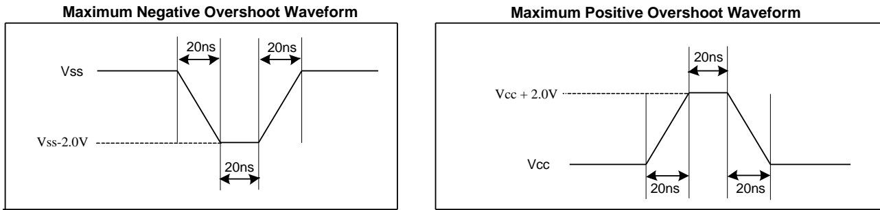
Figure 124 Input Test Waveform and Measurement Level
