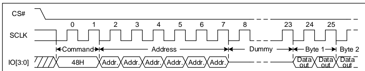
Figure 103 Read Security Registers command Sequence Diagram (QPI)
