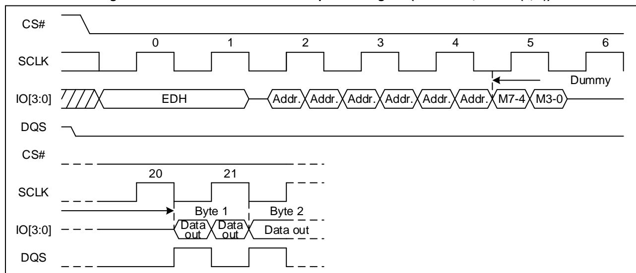
Figure 56. DTR Quad I/O Fast Read Sequence Diagram (Quad DTR, M5-4 ≠ (1, 0))
