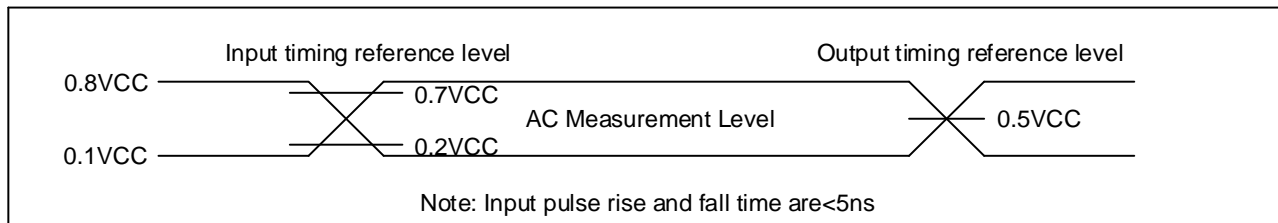
Figure 125 Input Test Waveform and Measurement Level
