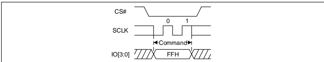
Figure 80 Disable QPI mode command Sequence Diagram (QPI & Quad DTR)
