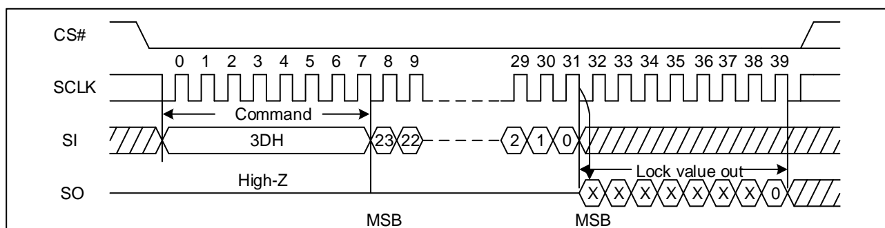
Figure 111 Read Individual Block/Sector lock command Sequence Diagram (SPI)
