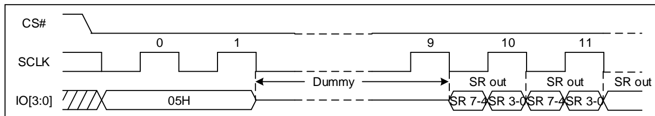
Figure 30 Read Status Register Sequence Diagram (Quad DTR)
