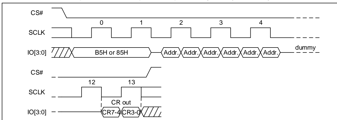
Figure 37 Read Configuration Registers Sequence (Quad DTR)
