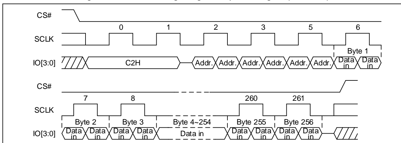
Figure 66 Extend Quad Page Program Sequence Diagram (Quad DTR)
