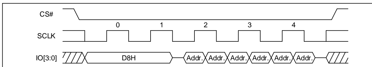
Figure 75 64KB Block Erase Sequence Diagram (Quad DTR)
