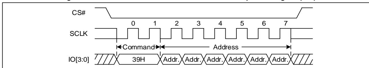
Figure 109 Individual Block/Sector Unlock command Sequence Diagram (QPI)
