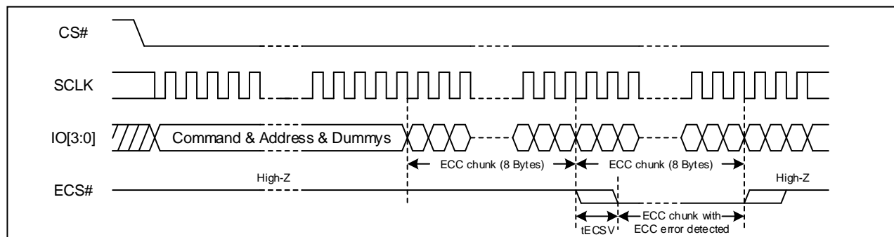
Figure 2. ECS# Timing
