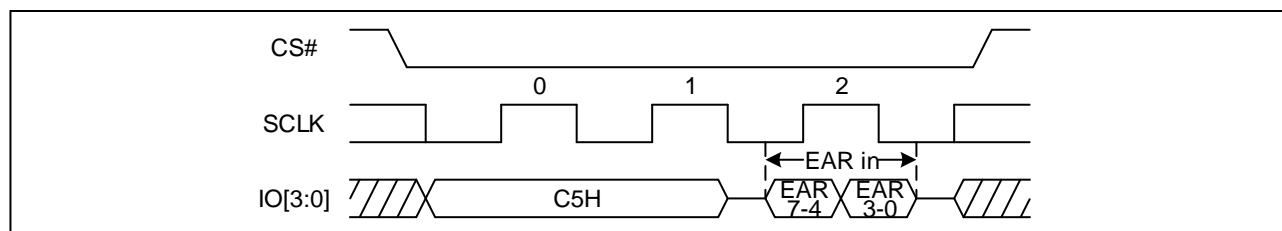
Figure 23 Write Extended Register Sequence Diagram (DTR, QPI)
