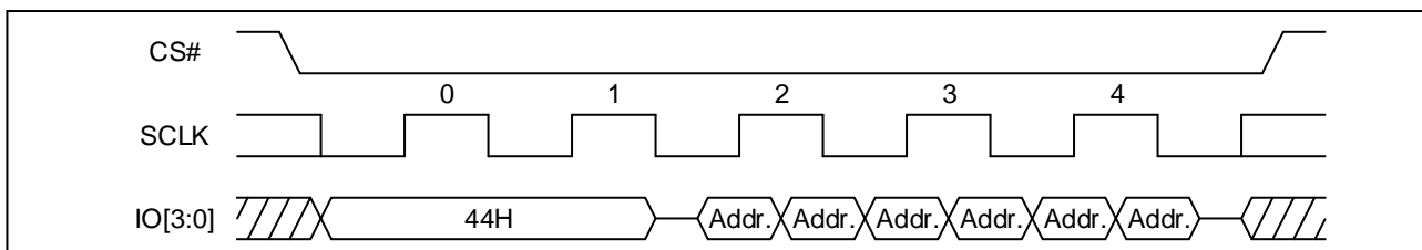
Figure 98 Erase Security Registers command Sequence Diagram (Quad DTR)
