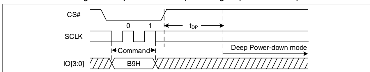
Figure 82 Deep Power-Down Sequence Diagram (QPI & Quad DTR)
