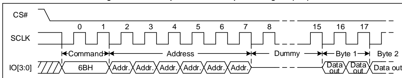
Figure 47 Quad Output Fast Read Sequence Diagram (QPI)
