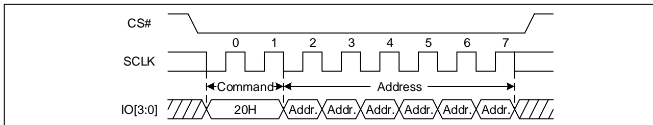
Figure 68 Sector Erase Sequence Diagram (QPI)
