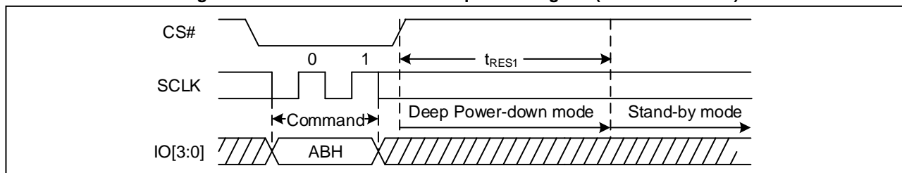
Figure 84 Release Power-Down Sequence Diagram (QPI &amp; Quad DTR)
