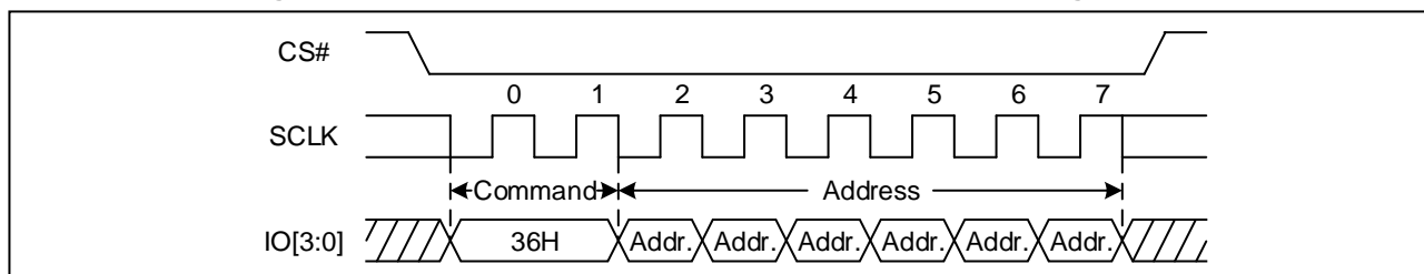
Figure 106 Individual Block/Sector Lock command Sequence Diagram (QPI)
