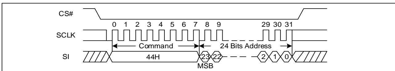
Figure 96 Erase Security Registers command Sequence Diagram (SPI)
