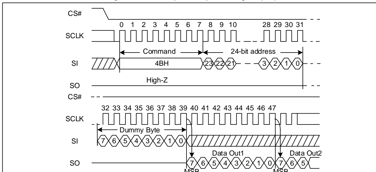
Figure 85 Read Unique ID Sequence Diagram (SPI)
