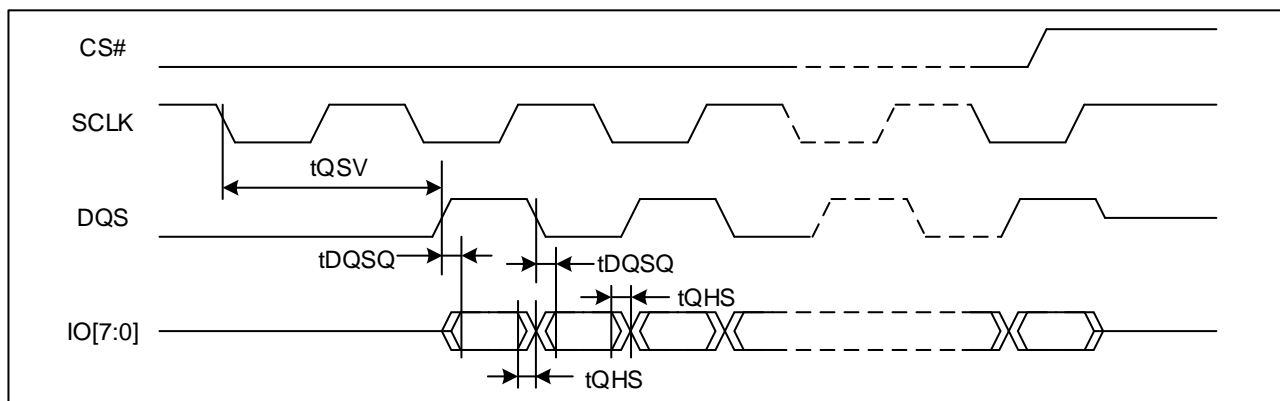
Figure 130. DQS Output Timing (DTR)
