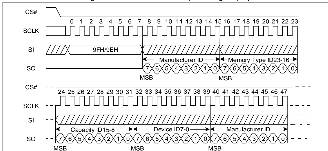
Figure 88 Read Identification ID Sequence Diagram (SPI)
