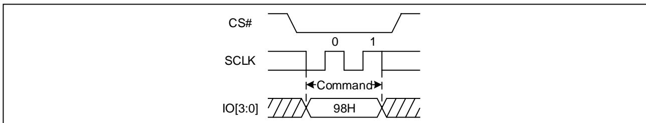
Figure 117 Global Block/Sector Unlock Sequence Diagram (QPI & Quad DTR)
