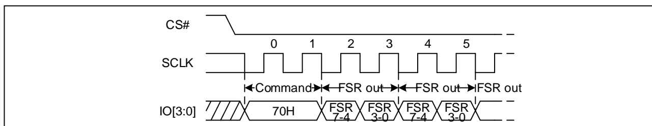
Figure 32 Read Flag Status Register Sequence Diagram (QPI, f_{SCLK} \leq 104\text{MHz} )
