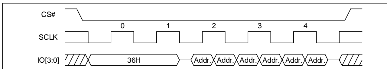
Figure 107 Individual Block/Sector Lock command Sequence Diagram (Quad DTR)
