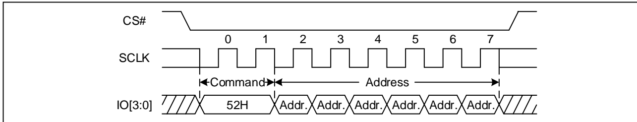
Figure 71 32KB Block Erase Sequence Diagram (QPI)
