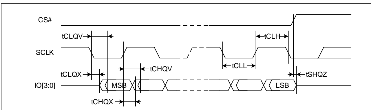
Figure 129. Serial Output Timing (DTR)
