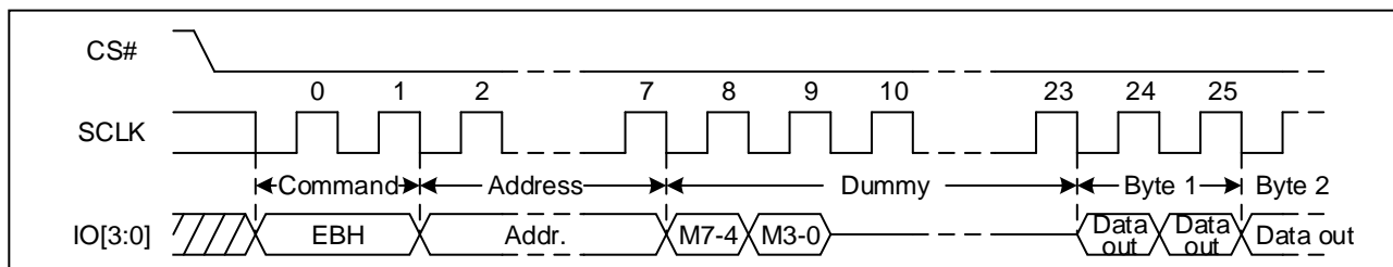
Figure 50 Quad I/O Fast Read Sequence Diagram (QPI, M5-4# (1, 0))
