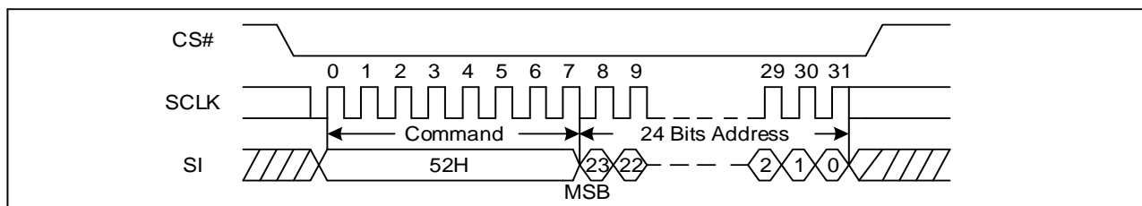
Figure 70 32KB Block Erase Sequence Diagram (SPI)
