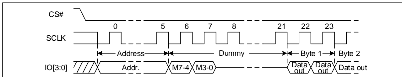
Figure 52 Quad I/O Fast Read Sequence Diagram (STR, M5-4= (1, 0))
