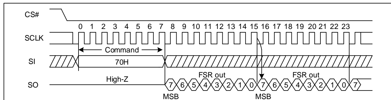
Figure 31 Read Flag Status Register Sequence Diagram (SPI)
