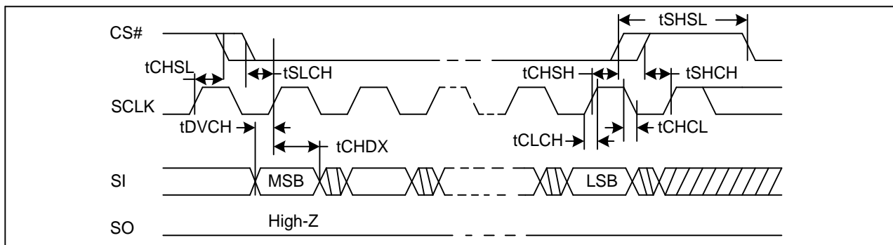
Figure 126 Serial Input Timing
