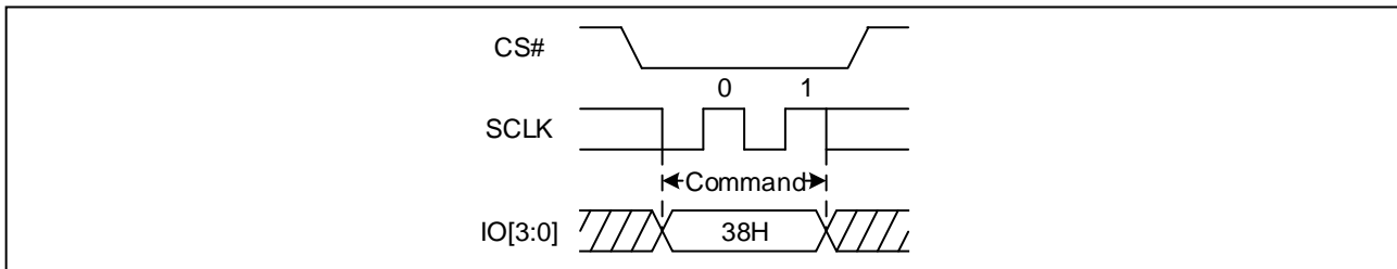
Figure 79 Enable QPI mode command Sequence Diagram (Quad DTR)
