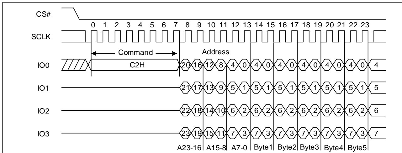
Figure 64 Extend Quad Page Program Sequence Diagram (SPI)
