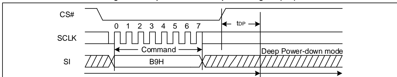
Figure 81 Deep Power-Down Sequence Diagram (SPI)
