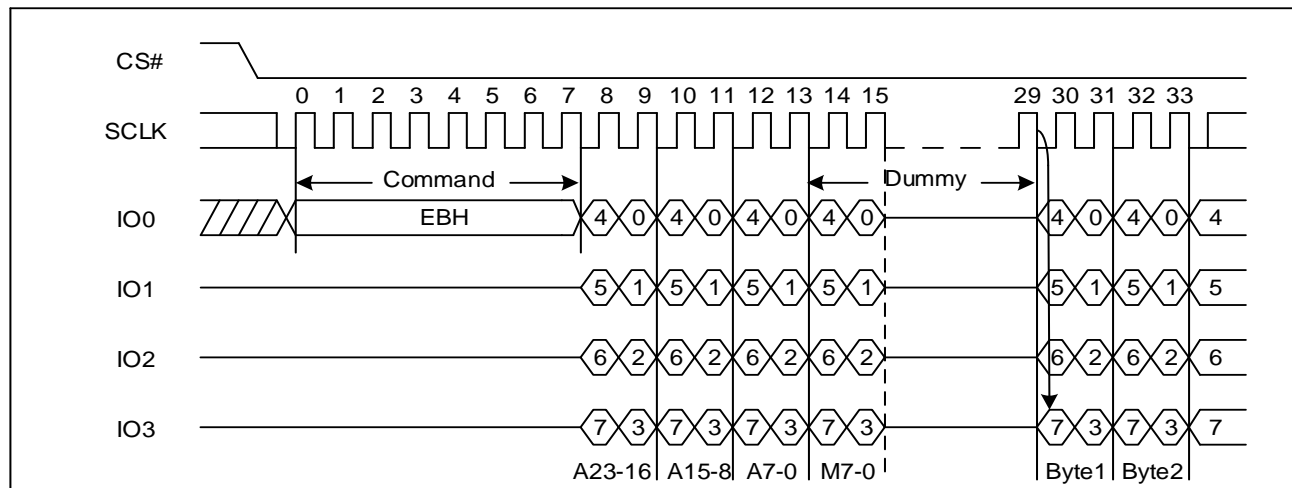
Figure 49 Quad I/O Fast Read Sequence Diagram (SPI, M5-4# (1, 0))
