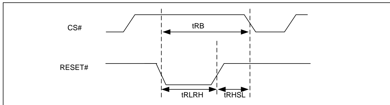
Figure 131 RESET Timing
