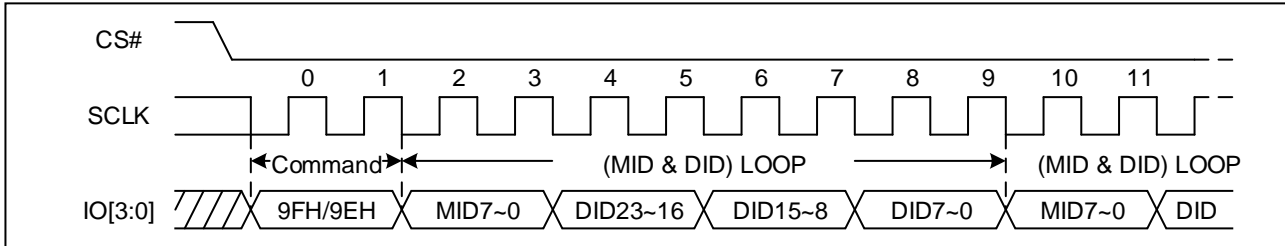
Figure 89 Read Identification ID Sequence Diagram (QPI, f_{SCLK} \leq 104\text{MHz} )
