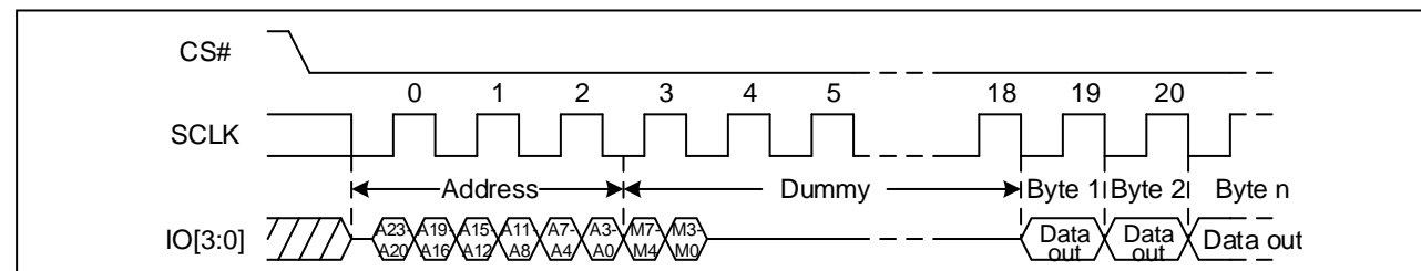
Figure 57. DTR Quad I/O Fast Read Sequence Diagram (M5-4 = (1, 0))
