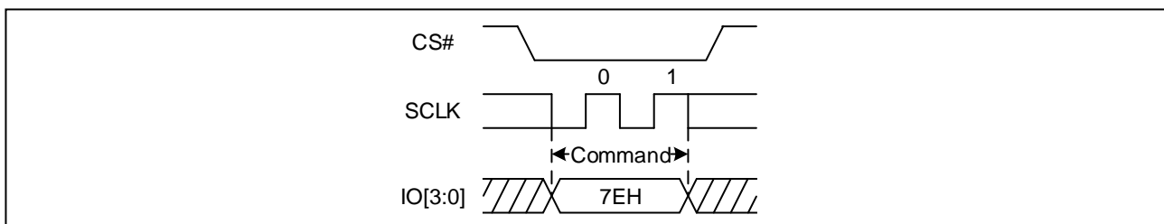
Figure 115 Global Block/Sector Lock Sequence Diagram (QPI & Quad DTR)
