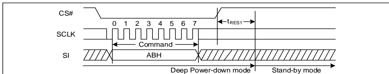
Figure 83 Release Power-Down Sequence Diagram (SPI)
