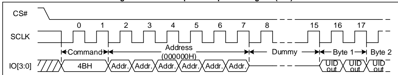
Figure 86 Read Unique ID Sequence Diagram (QPI)
