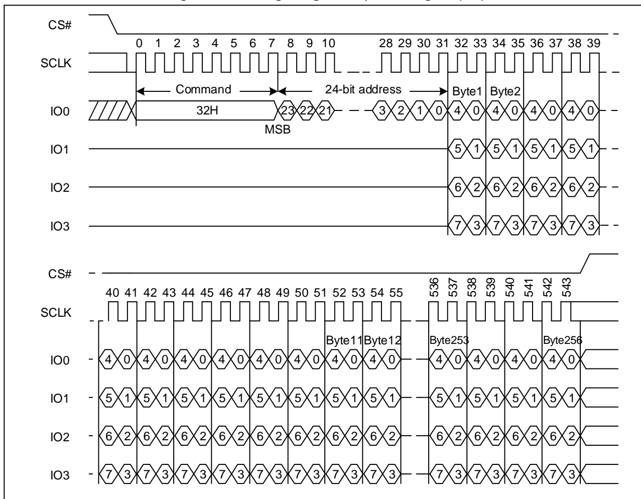
Figure 61 Quad Page Program Sequence Diagram (SPI)
