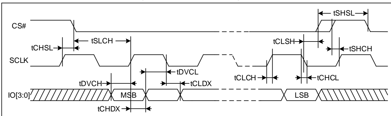
Figure 128. Serial Input Timing (DTR)
