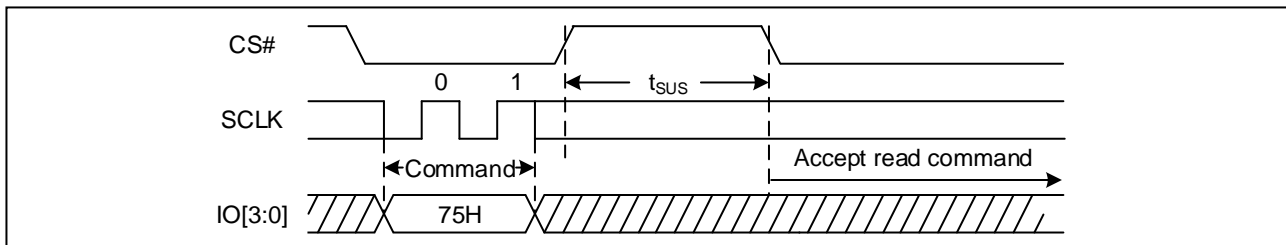
Figure 93 Program/Erase Suspend Sequence Diagram (QPI & Quad DTR)
