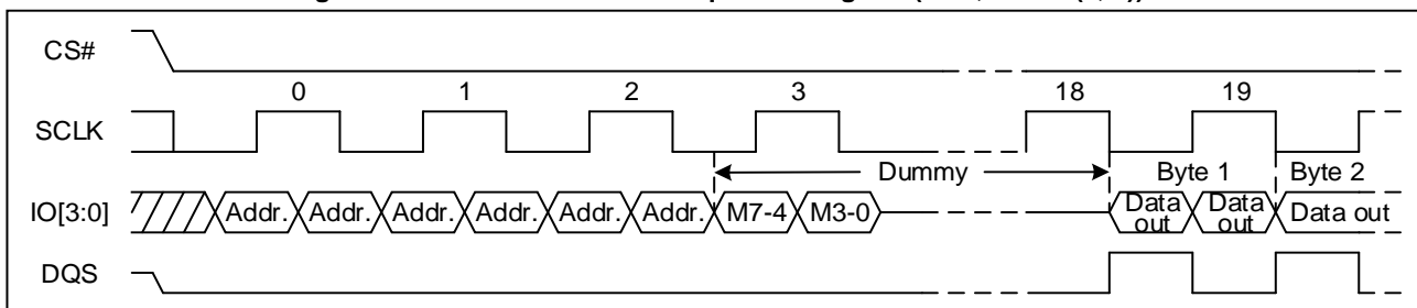
Figure 53 Quad I/O Fast Read Sequence Diagram (DTR, M5-4= (1, 0))
