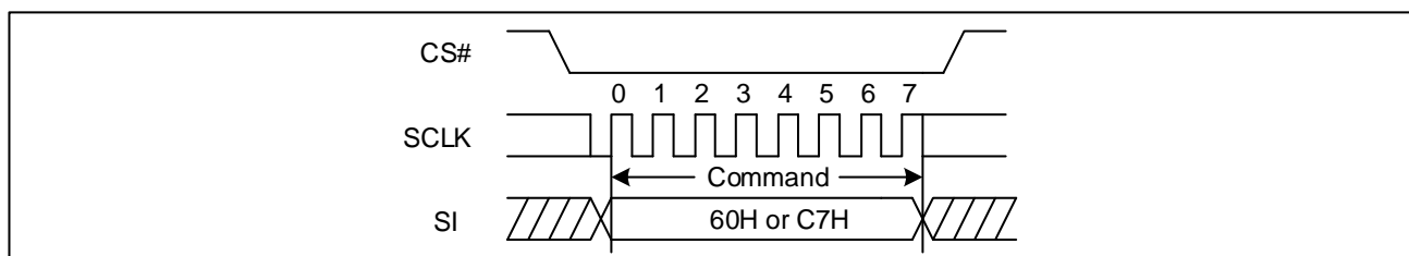
Figure 76 Chip Erase Sequence Diagram (SPI)
