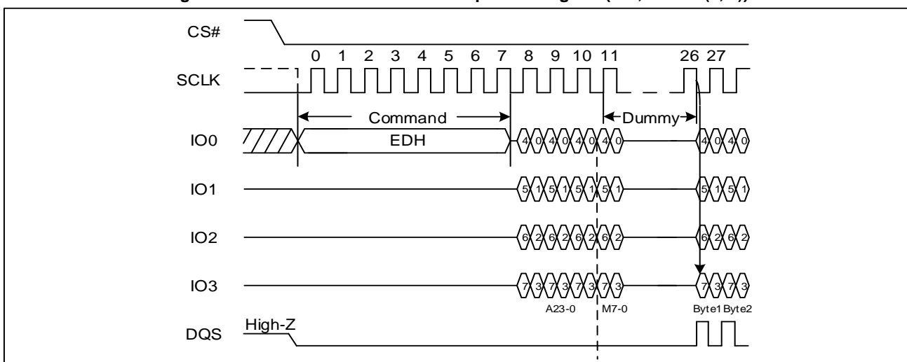
Figure 54. DTR Quad I/O Fast Read Sequence Diagram (SPI, M5-4 ≠ (1, 0))
