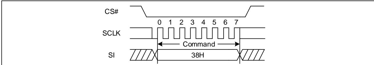
Figure 78 Enable QPI mode command Sequence Diagram (SPI)
