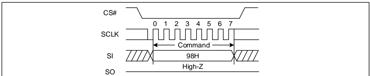
Figure 116 Global Block/Sector Unlock Sequence Diagram (SPI)
