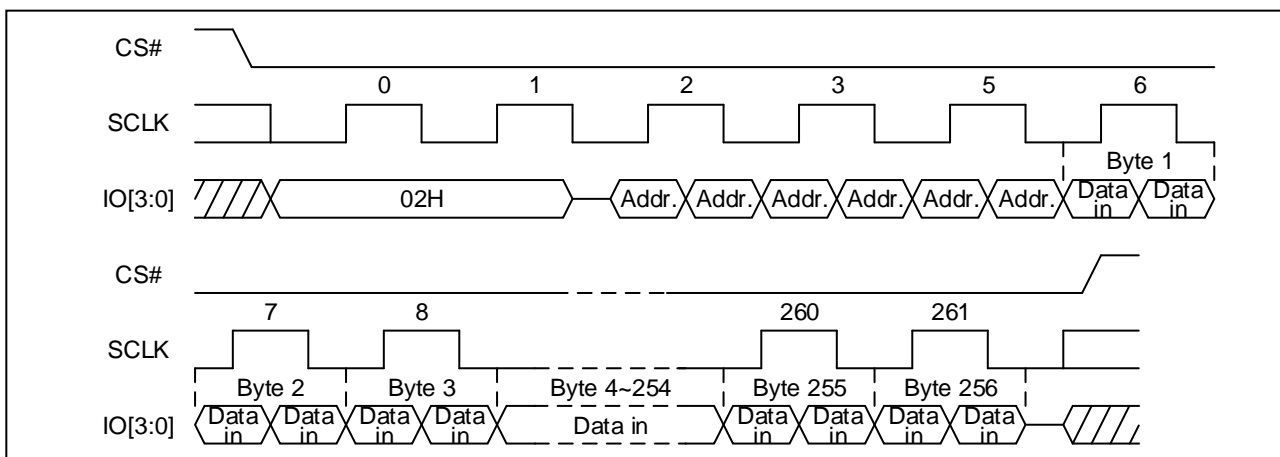
Figure 60 Page Program Sequence Diagram (Quad DTR)
