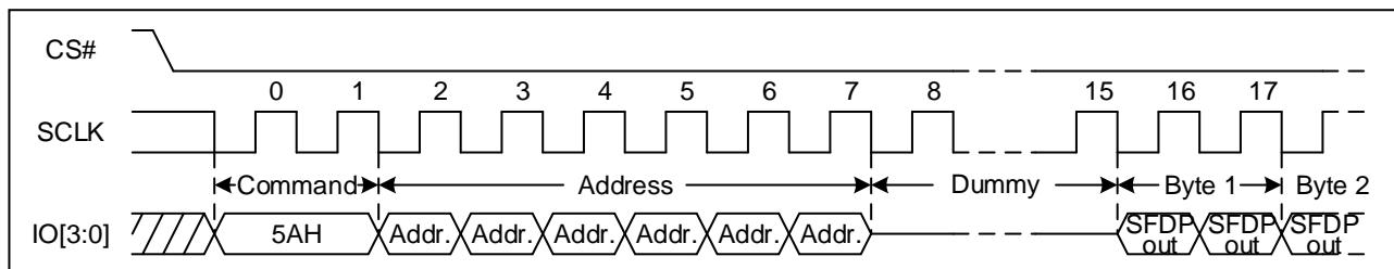
Figure 121 Read Serial Flash Discoverable Parameter command Sequence Diagram (QPI)
