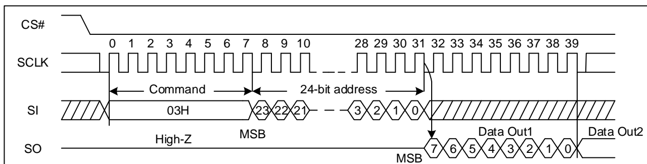
Figure 42 Read Data Bytes Sequence Diagram
