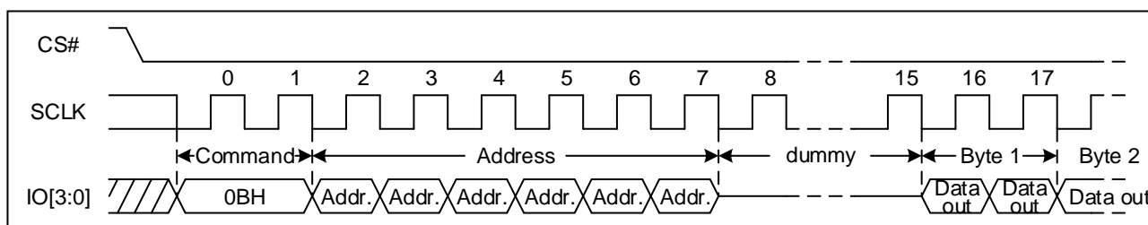
Figure 44 Read Data Bytes at Higher Speed Sequence Diagram (QPI)
