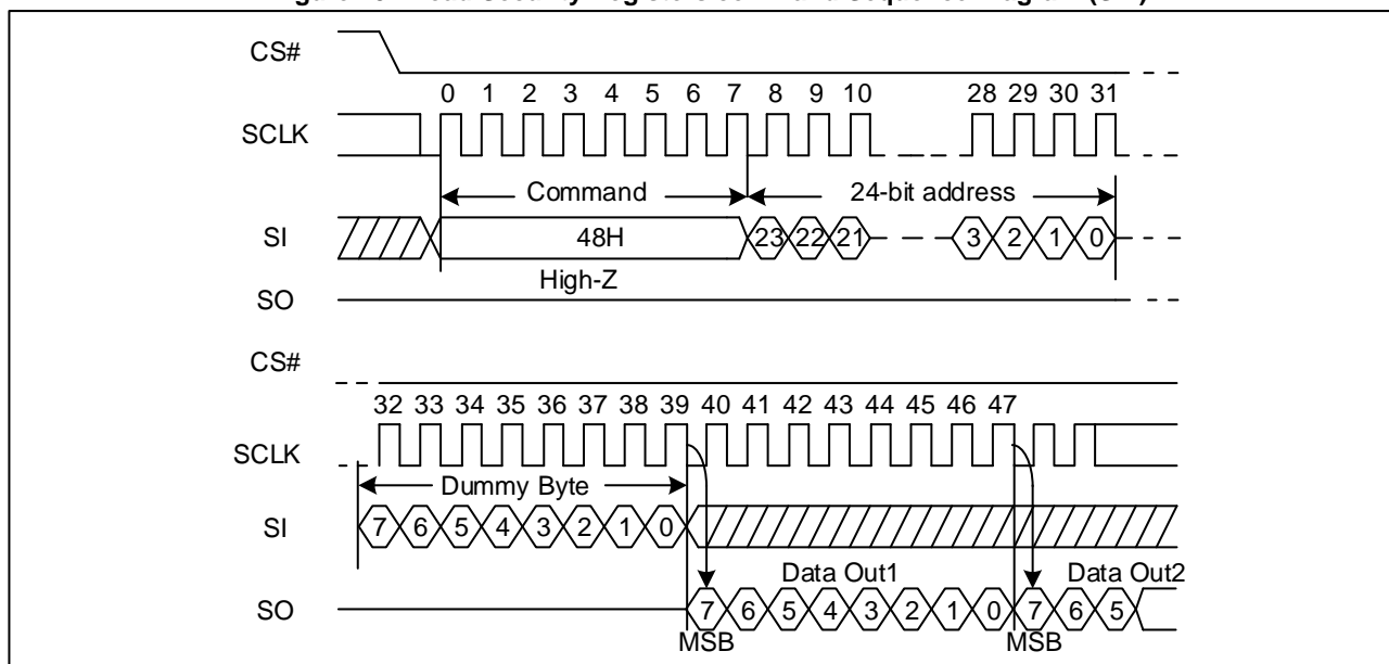
Figure 102 Read Security Registers command Sequence Diagram (SPI)
