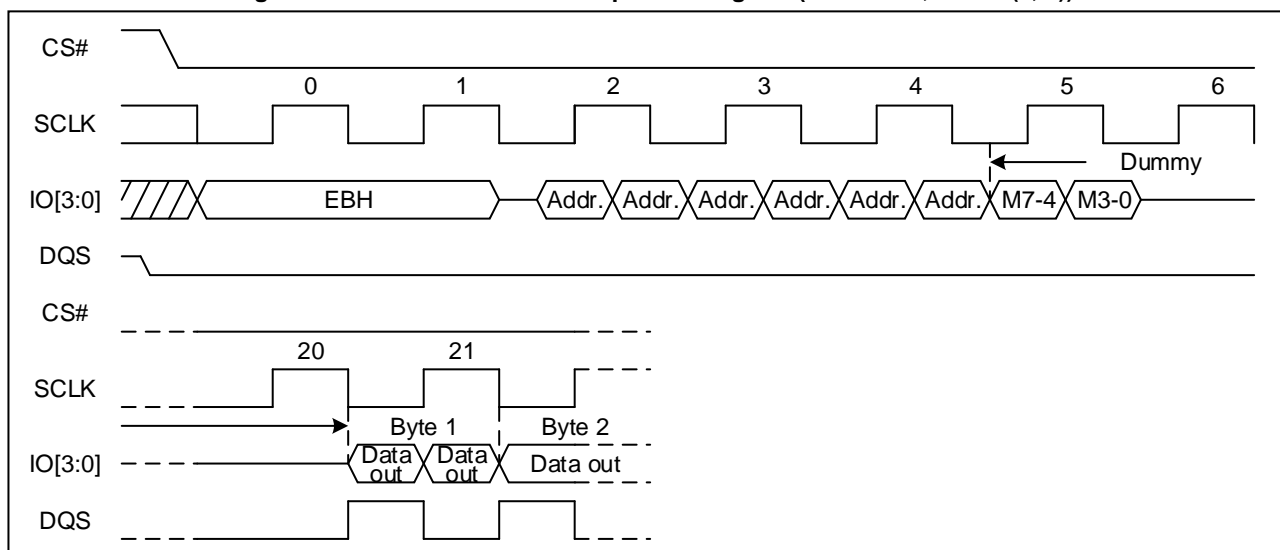
Figure 51 Quad I/O Fast Read Sequence Diagram (Quad DTR, M5-4# (1, 0))
