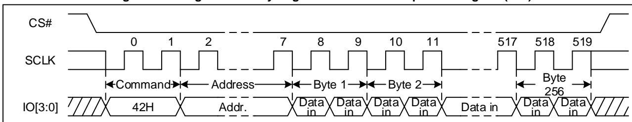
Figure 100 Program Security Registers command Sequence Diagram (QPI)
