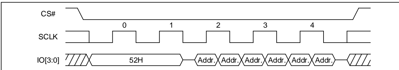
Figure 72 32KB Block Erase Sequence Diagram (Quad DTR)
