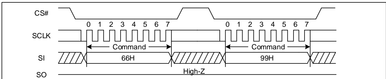
Figure 118 Enable Reset and Reset command Sequence Diagram (SPI)
