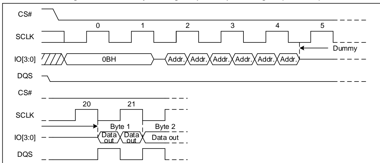
Figure 45 Read Data Bytes at Higher Speed Sequence Diagram (Quad DTR)
