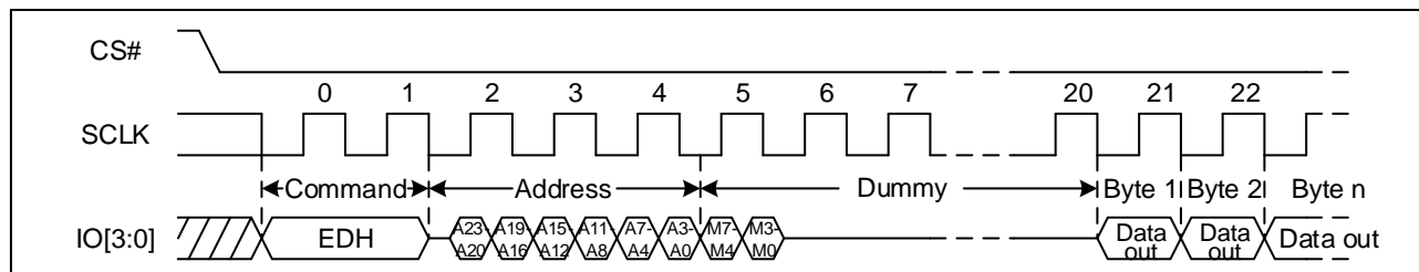
Figure 55. DTR Quad I/O Fast Read Sequence Diagram (QPI, M5-4 ≠ (1, 0))
