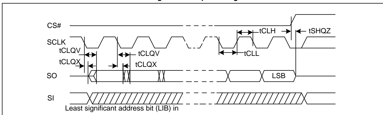
Figure 127 Output Timing
