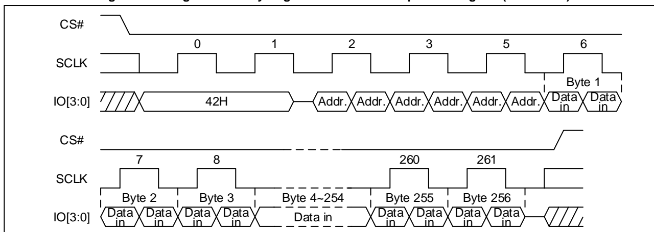
Figure 101 Program Security Registers command Sequence Diagram (Quad DTR)
