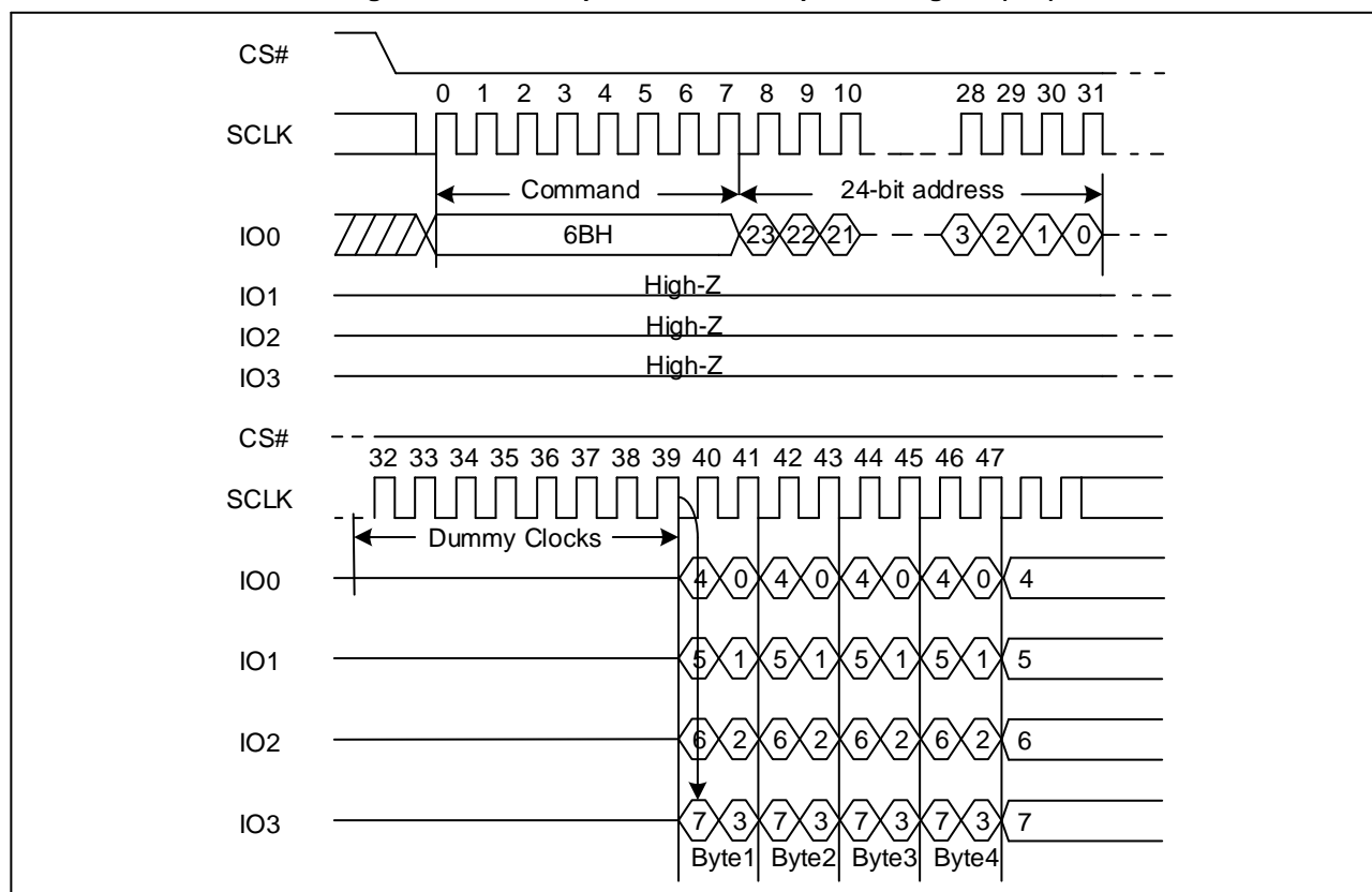
Figure 46 Quad Output Fast Read Sequence Diagram (SPI)
