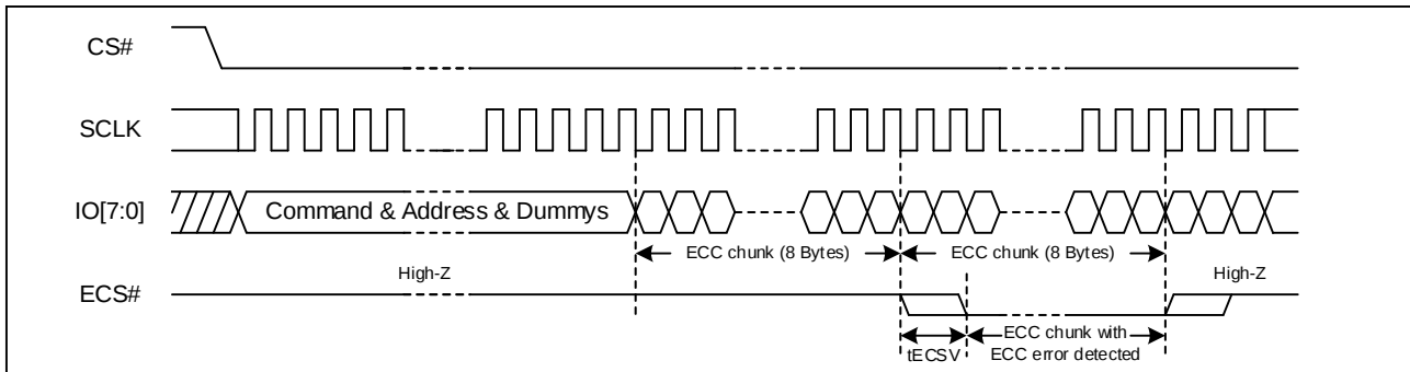
Figure 2. ECS# Timing
