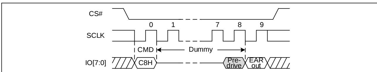
Figure 35. Read Extended Register Sequence Diagram (STR OPI)
