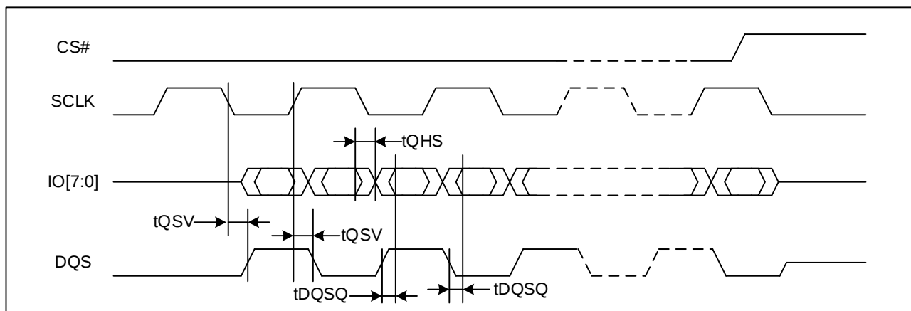
Figure 121. DQS Output Timing (DTR)
