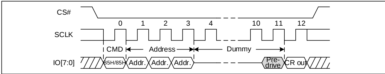
Figure 32. Read Configuration Registers Sequence (STR OPI)
