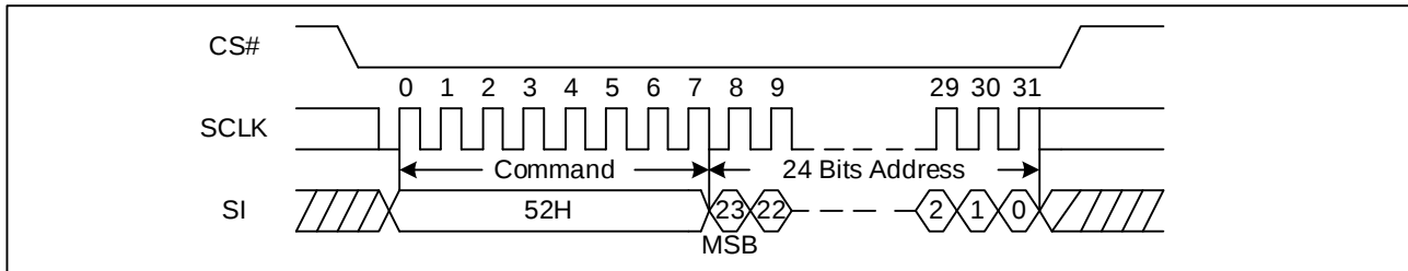
Figure 63. 32KB Block Erase Sequence Diagram (SPI)
