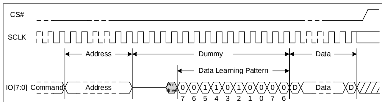
Figure 4. Data Learning Pattern Sequence Diagram (STR, Dummy Clock \geq 12 )
