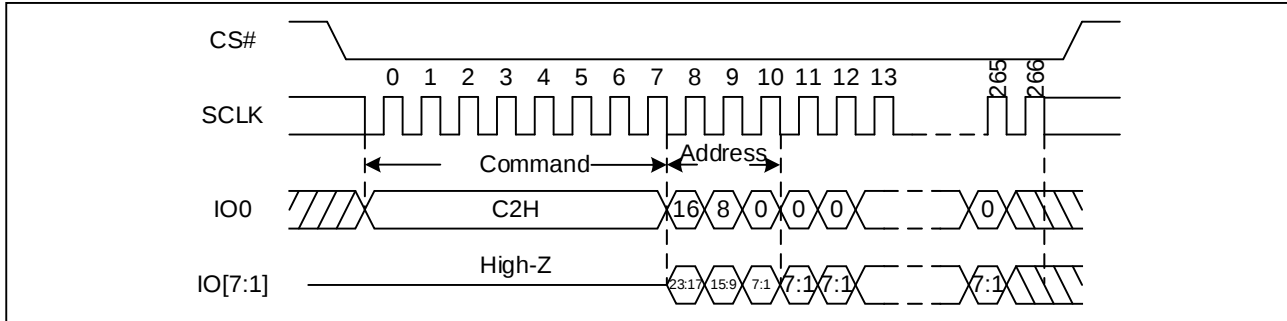
Figure 57. Extend Octal Page Program Sequence Diagram (SPI)
