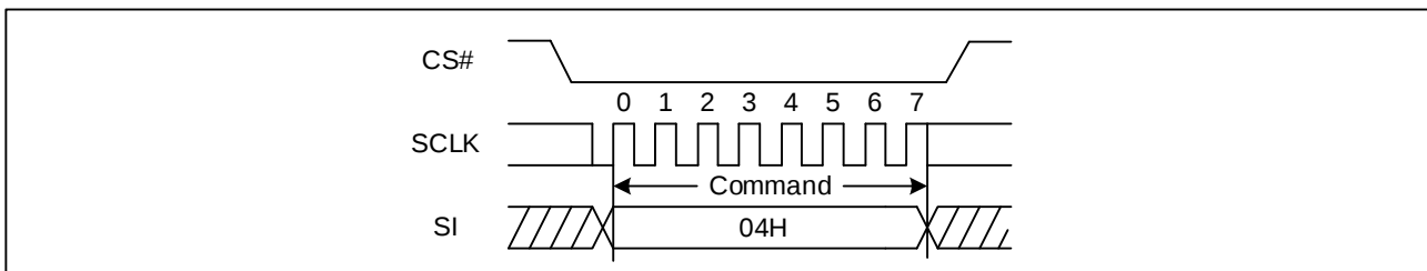
Figure 14. Write Disable Sequence Diagram (SPI)
