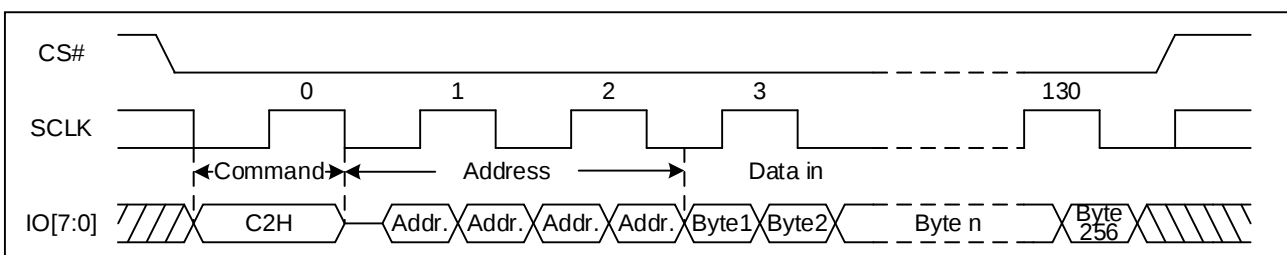
Figure 59. Page Program Sequence Diagram (DTR OPI)
