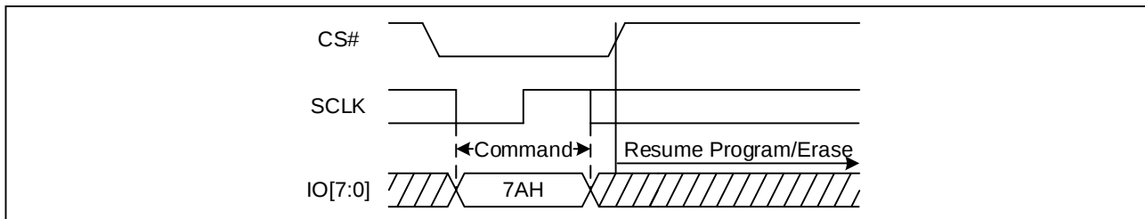
Figure 86. Program/Erase Resume Sequence Diagram (OPI)
