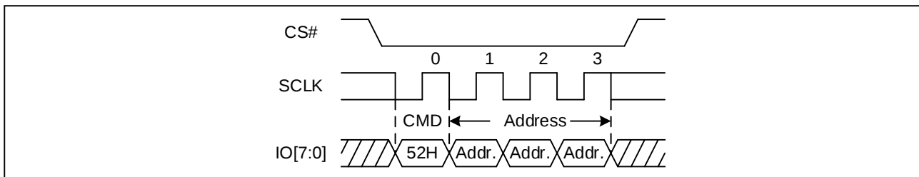
Figure 64. 32KB Block Erase Sequence Diagram (STR OPI)
