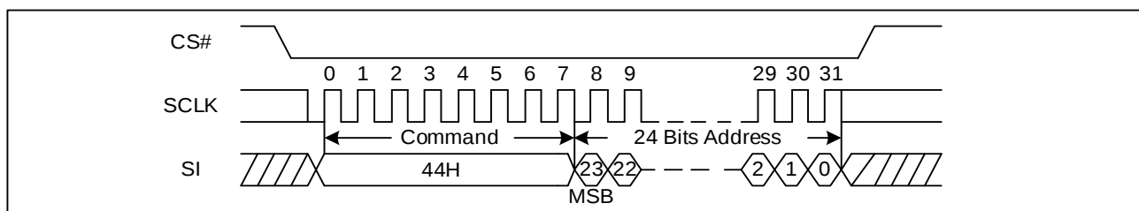
Figure 87. Erase Security Registers command Sequence Diagram (SPI)
