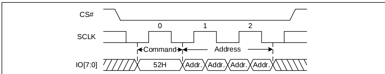
Figure 65. 32KB Block Erase Sequence Diagram (DTR OPI)
