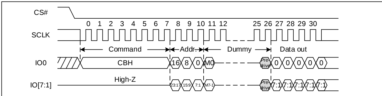
Figure 44. Octal I/O Fast Read Sequence Diagram (SPI, M5-4 \neq (1, 0))
