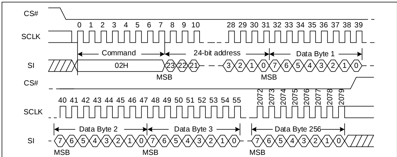
Figure 51. Page Program Sequence Diagram (SPI)
