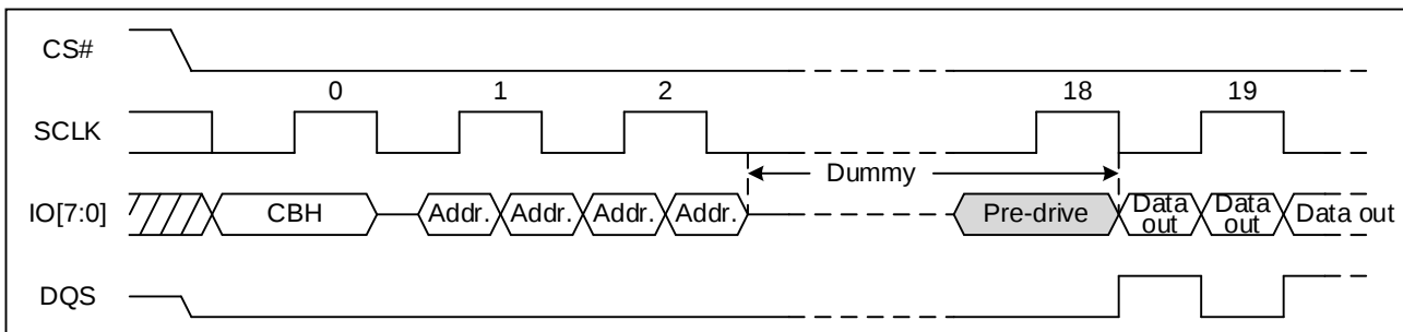
Figure 46. Octal Output Fast Read Sequence Diagram (DTR OPI, M5-4 \neq (1, 0))
