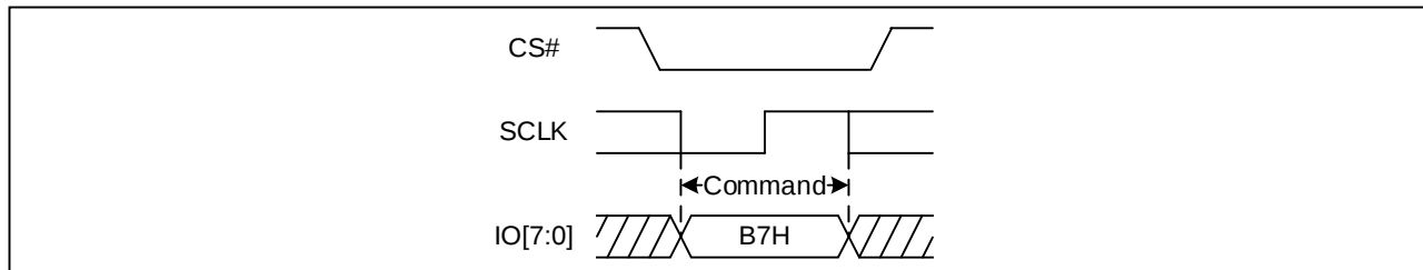
Figure 9. Enable 4-byte Mode Sequence Diagram (OPI)
