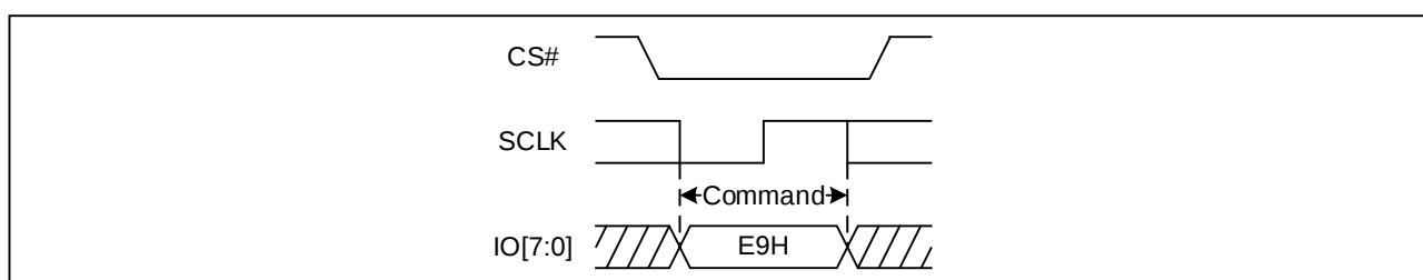
Figure 11. Disable 4-byte Mode Sequence Diagram (OPI)
