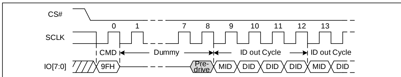
Figure 81. Read Identification ID Sequence Diagram (STR, OPI)
