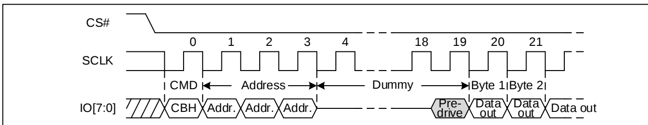
Figure 45. Octal I/O Fast Read Sequence Diagram (STR OPI, M5-4 \neq (1, 0))
