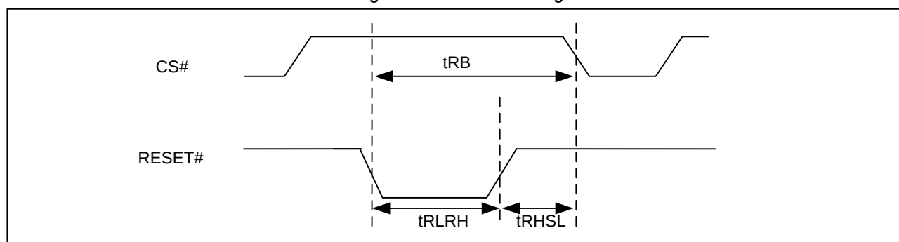
Figure 122. RESET Timing
