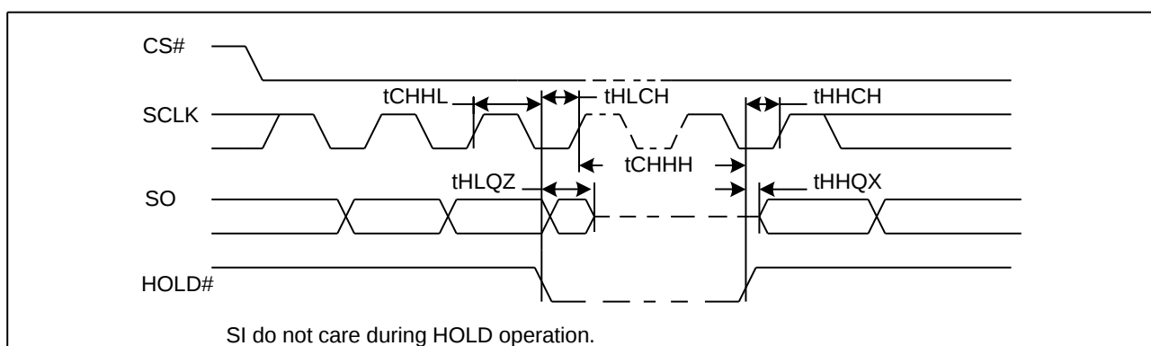
Figure 43. Hold Timing
