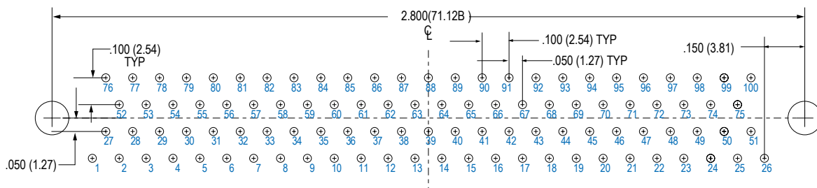
100 SOCKET M83513/27-H
