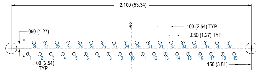
37 SOCKET M83513/25-F
