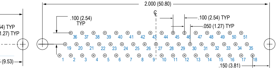
51 SOCKET M83513/26-G
