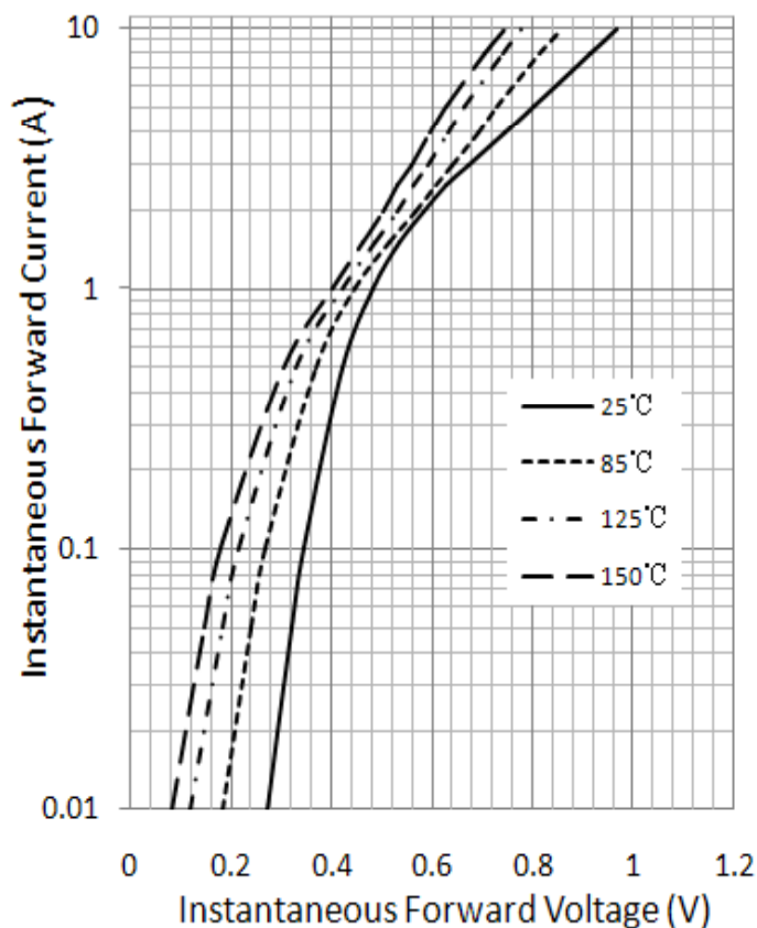
Figure 4. Typical Instantaneous Forward Characteristics
