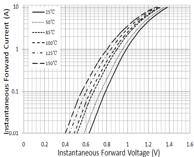
Figure 4. Typical Instantaneous Forward Characteristics
