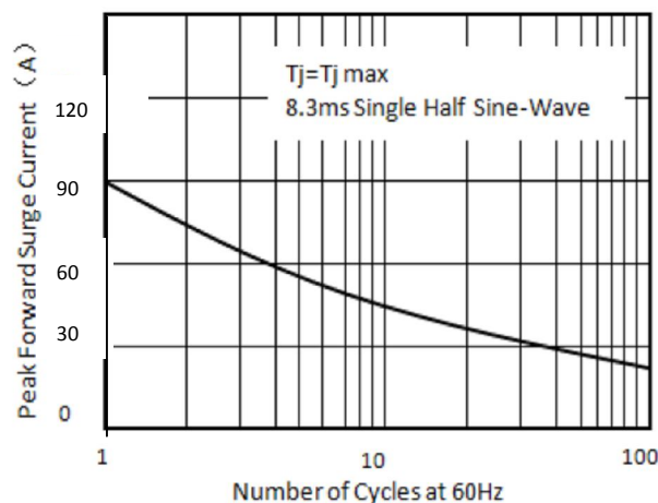
Figure 4. Maximum Non-Repertive Peak Forward Surge Current
