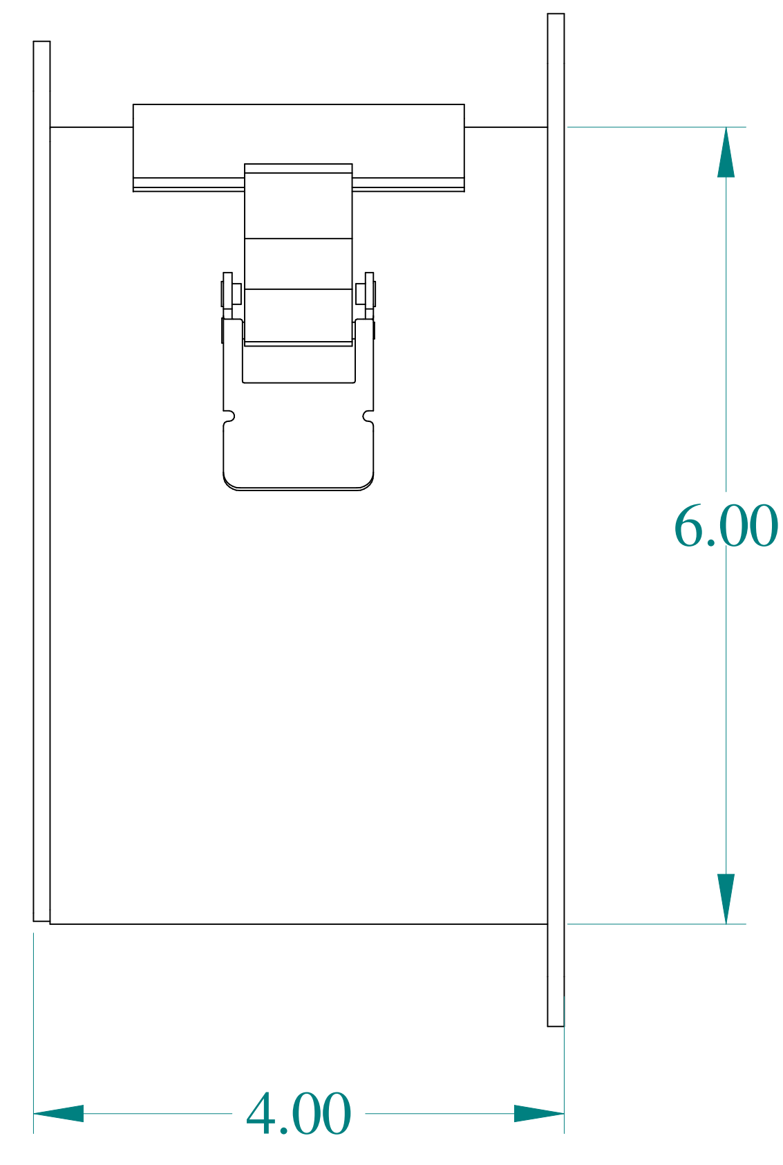
FRONT VIEW
