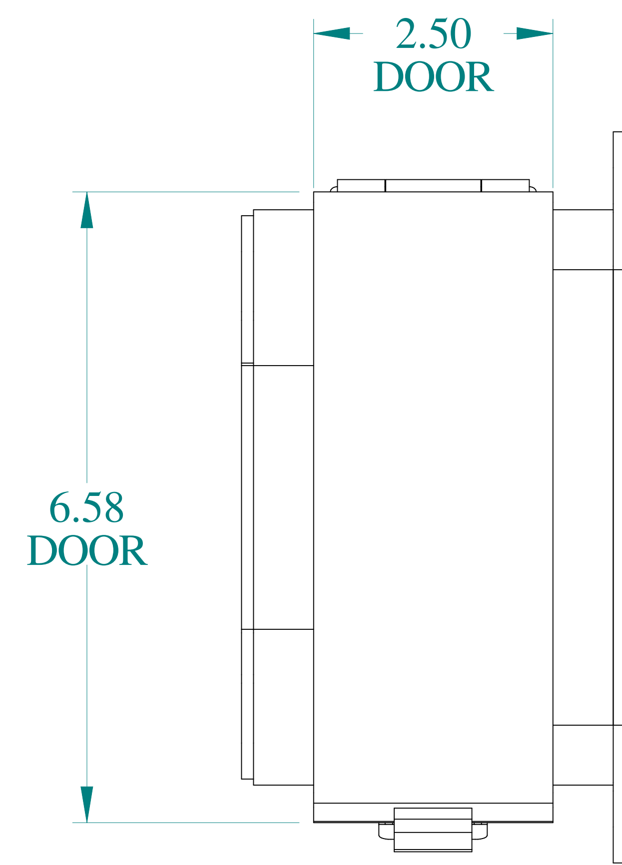
TOP VIEW
