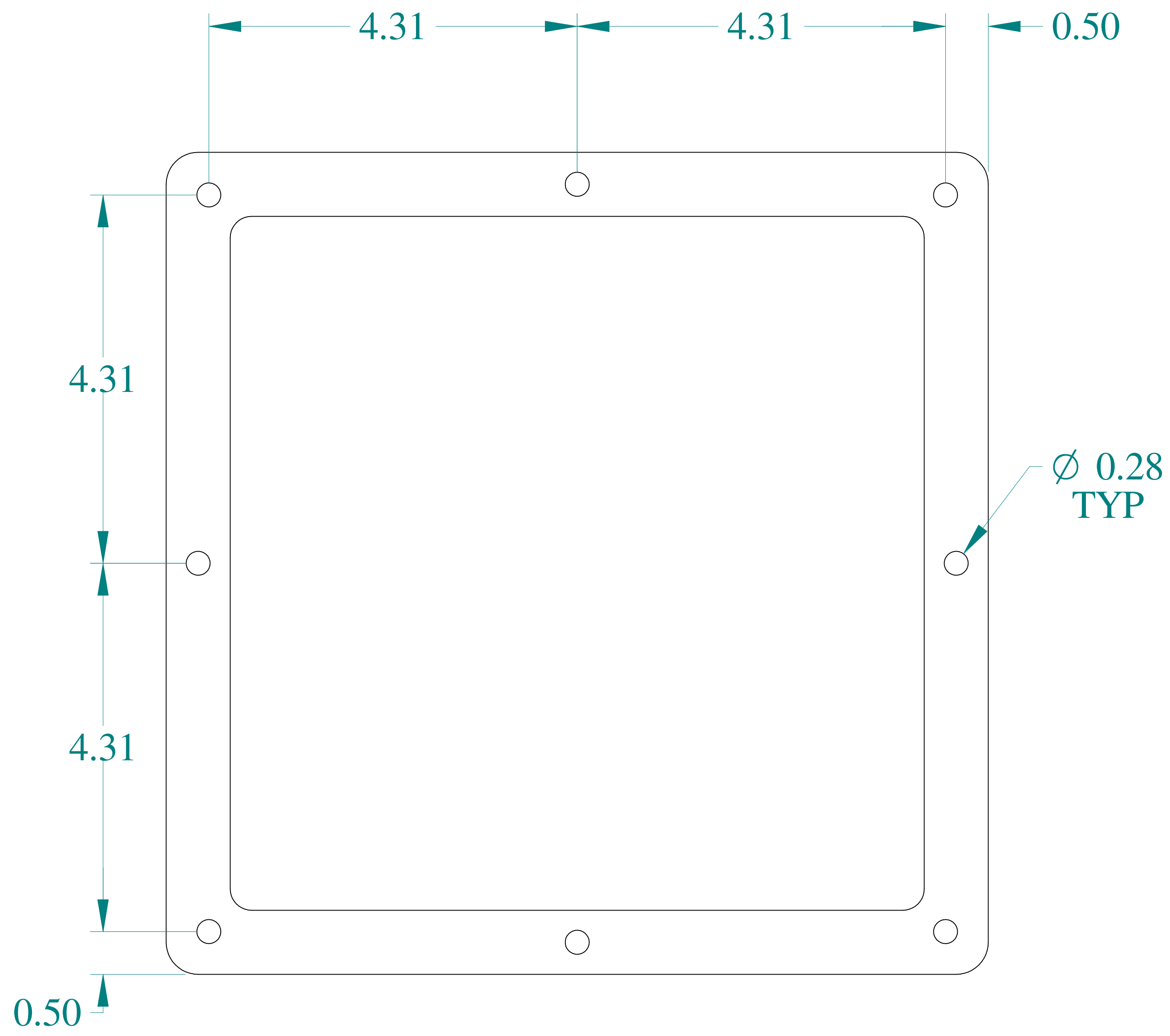
FRONT VIEW
