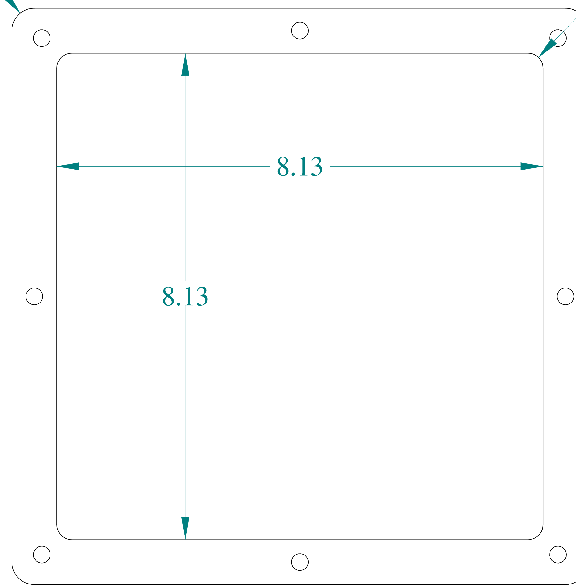
BACK VIEW
